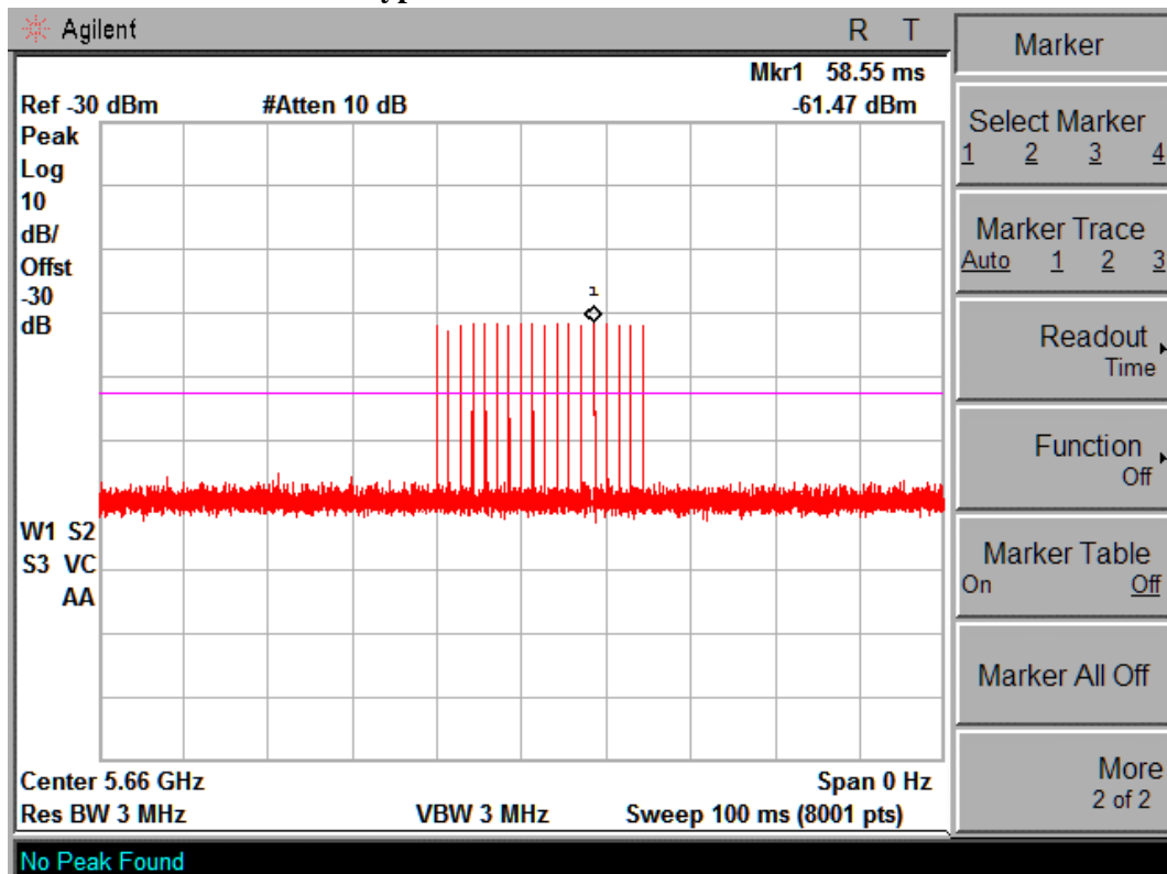
Radar Type 1 Calibration Plot 5660MHz
