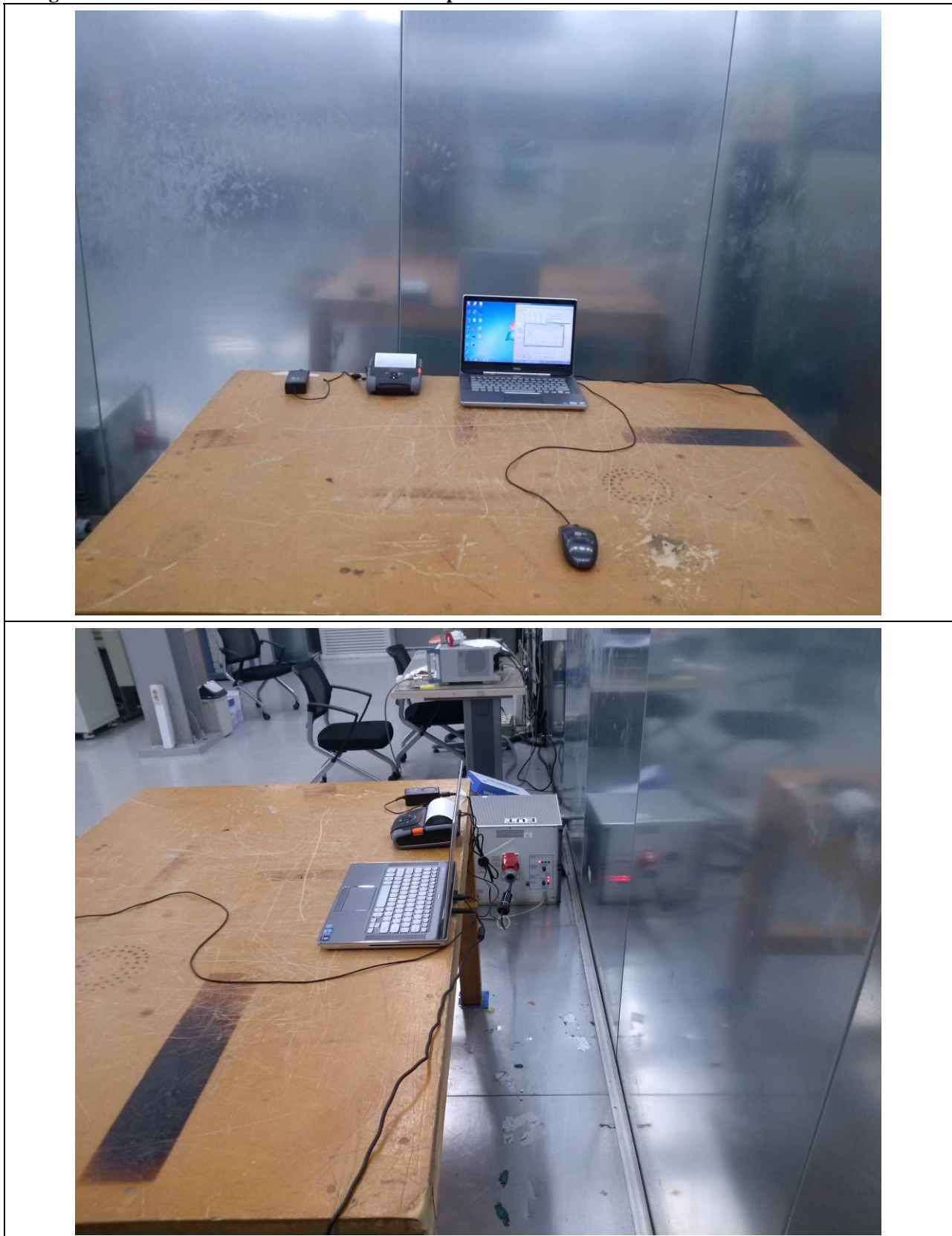
Figure 3. Photo of Conducted Emission Test Setup
