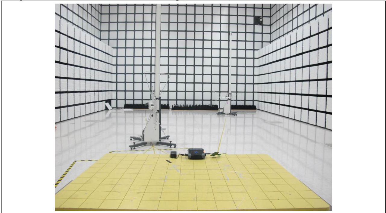
Figure 1. Photo of Radiated Emission Test Setup (below 1 GHz)
