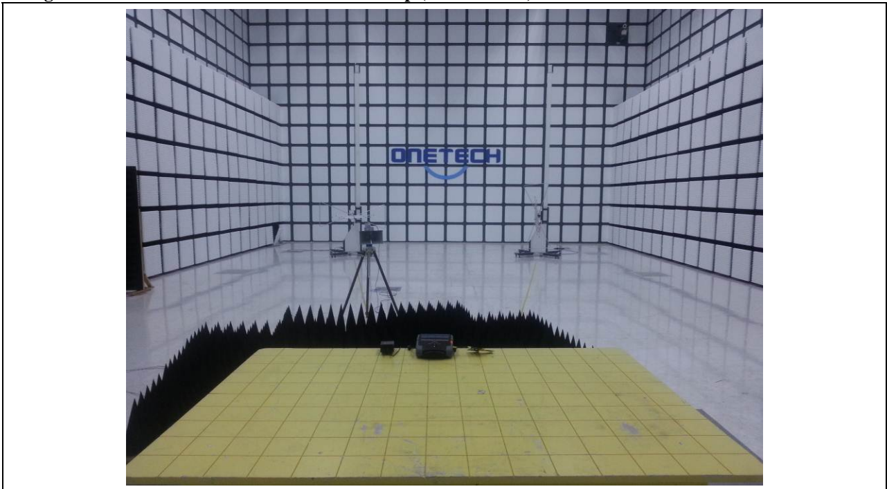
Figure 2. Photo of Radiated Emission Test Setup (above 1 GHz)
