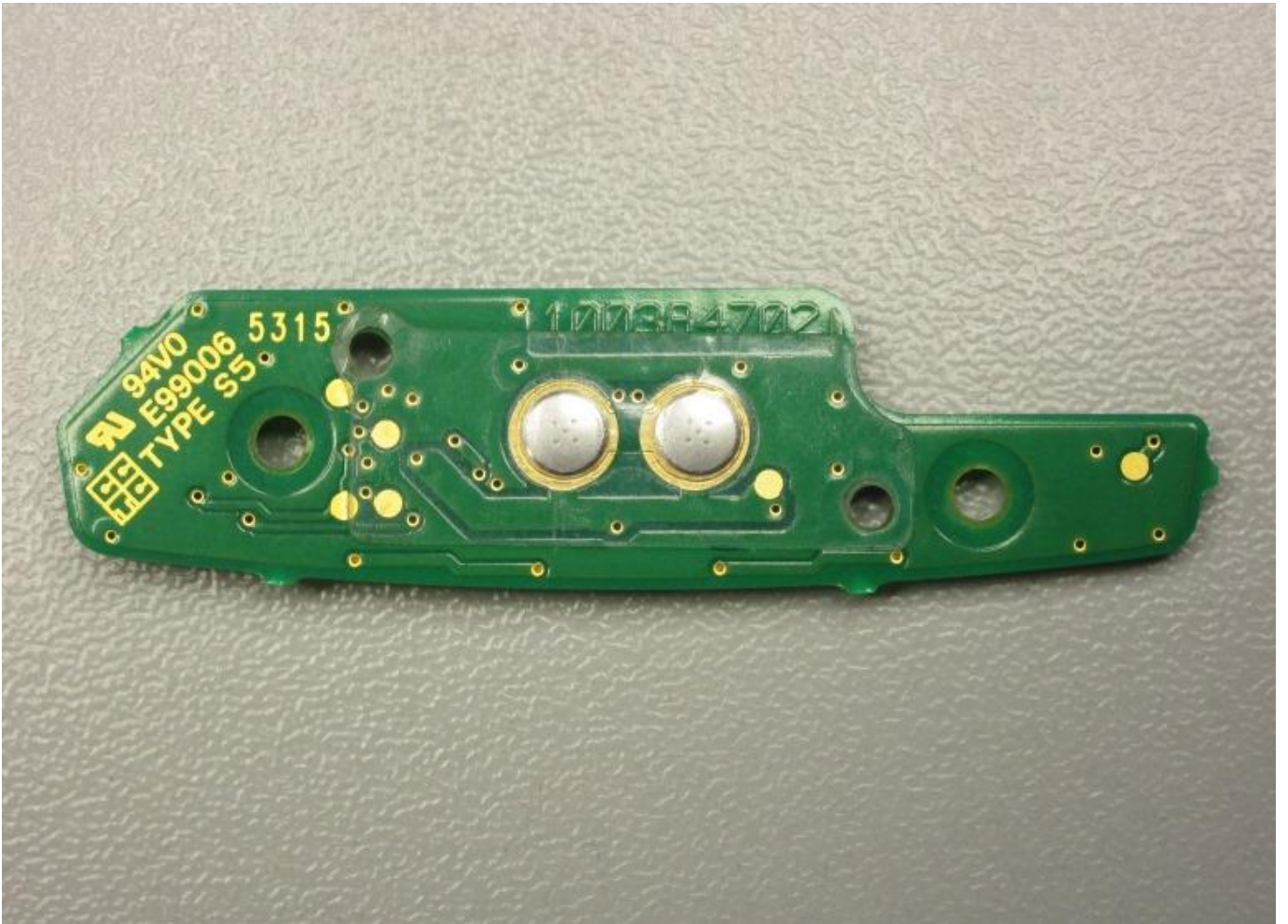
HOME_KEY/LED Board (Top)
