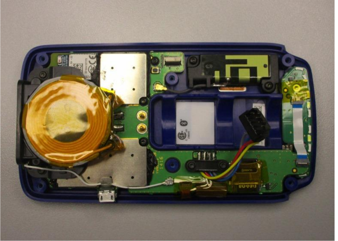
Internal Overview
