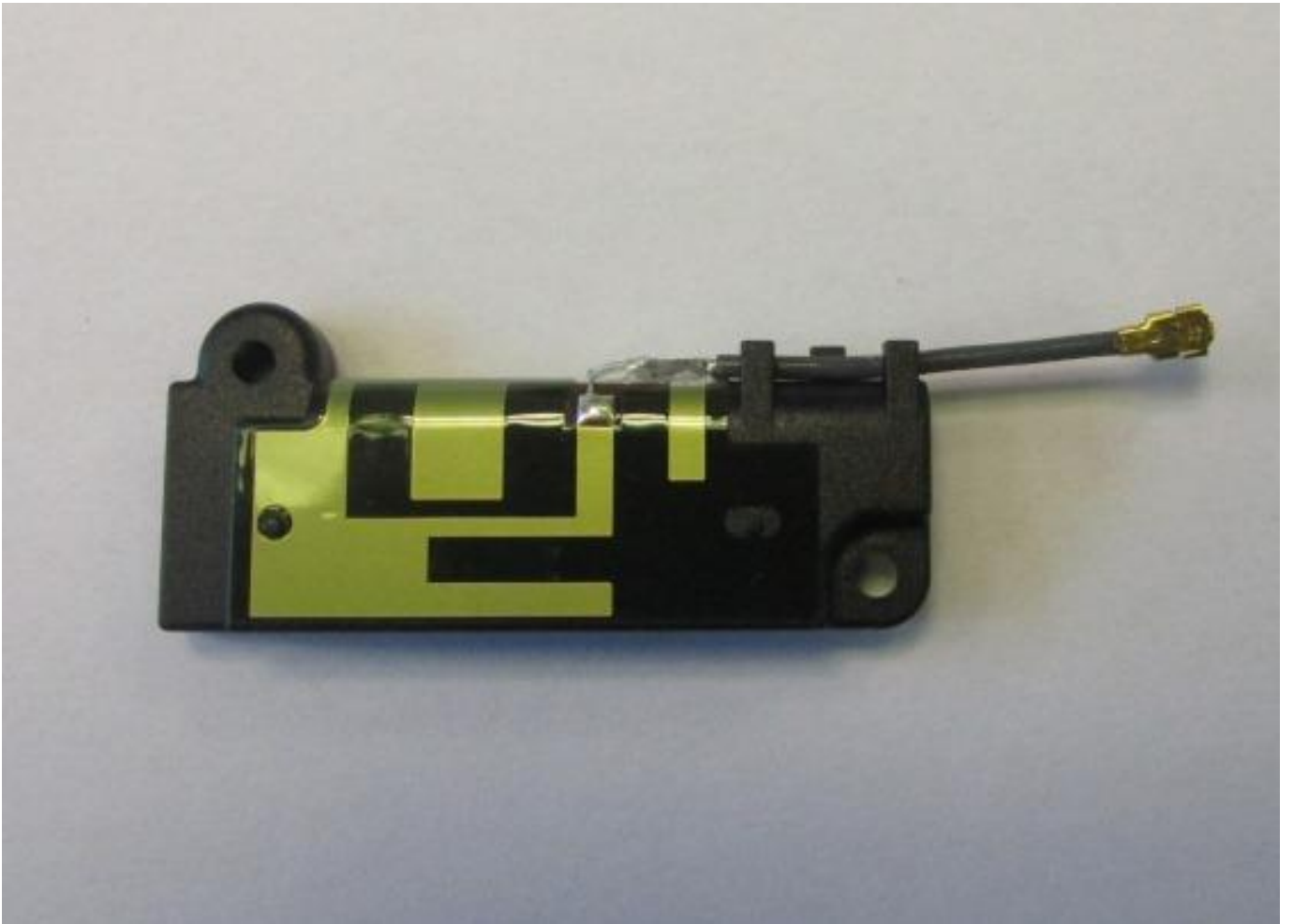
WLAN Antenna
