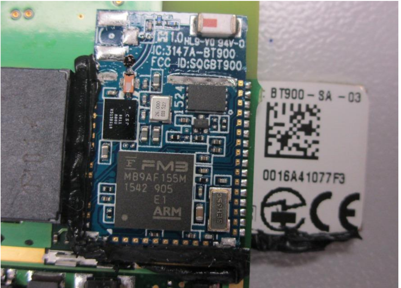
Bluetooth module and Antenna
