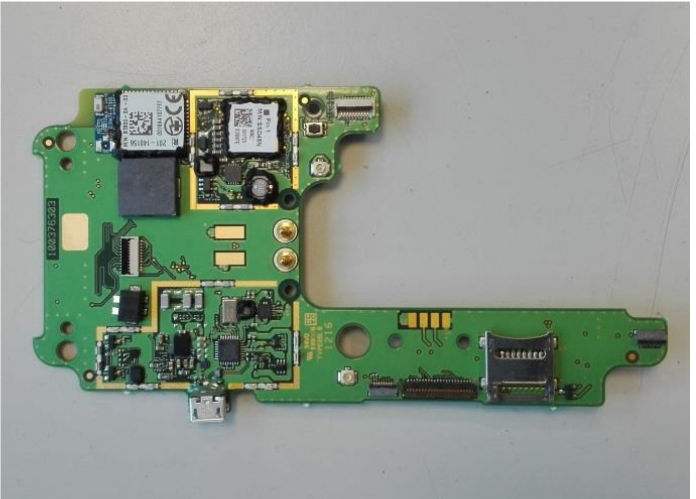
Mainboard (Top)
