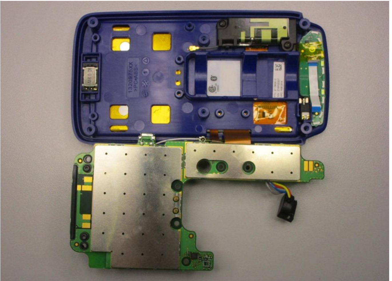
Internal Assembly
