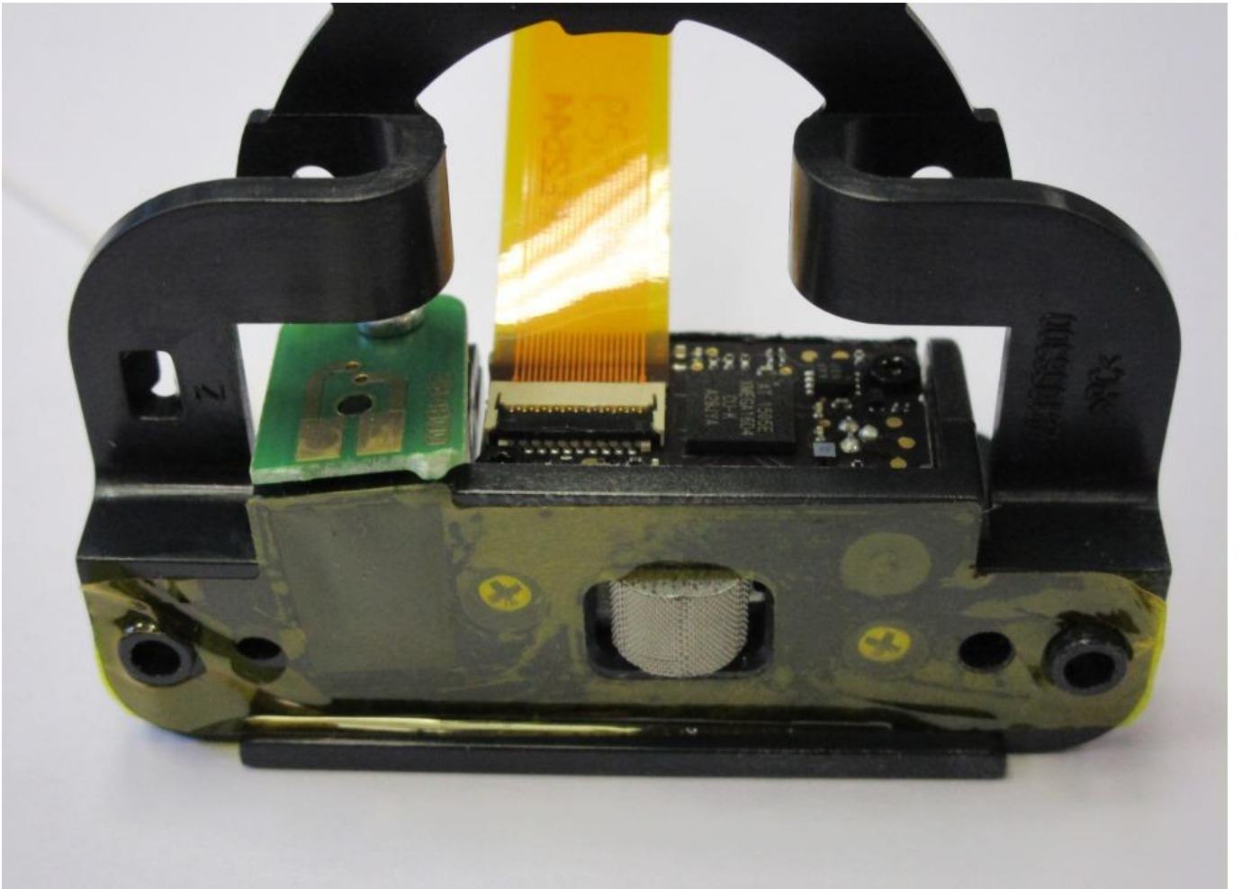
Reader Assembly
