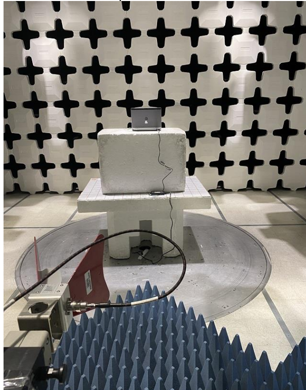
Setup 1-18 GHz Front
