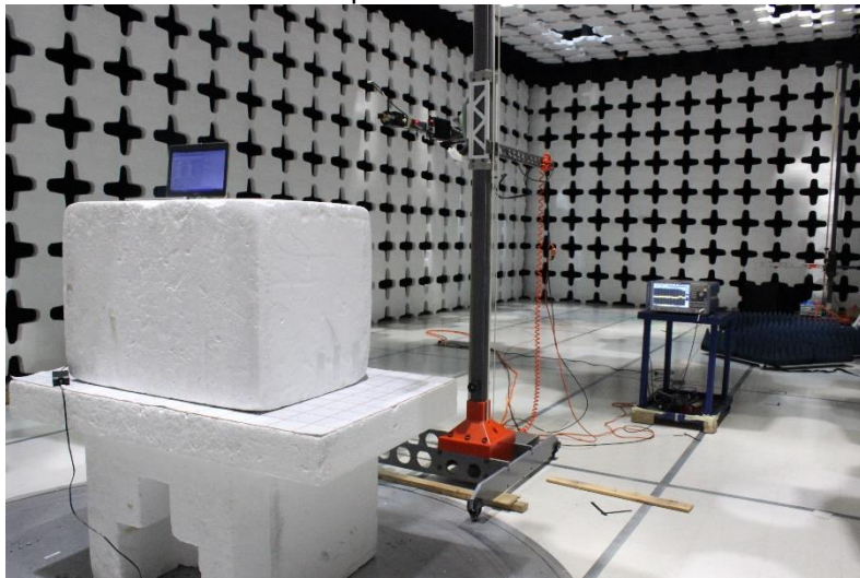
Setup 18-40 GHz Rear
