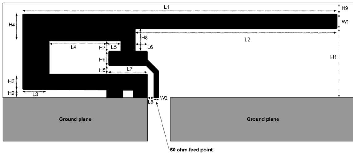
Figure 1-1. IFA Dimensions
