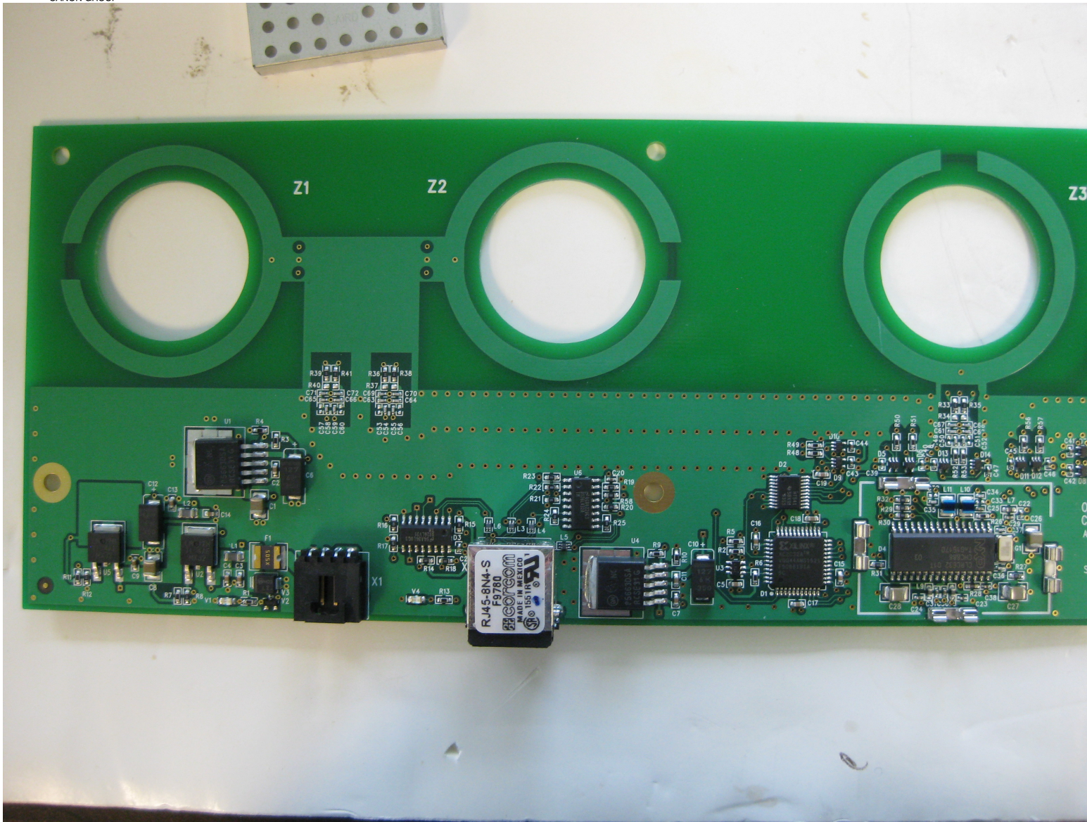
Figure 5: 3010120604 RFID Reader Front Left Side close up – RF Shield is removed.
