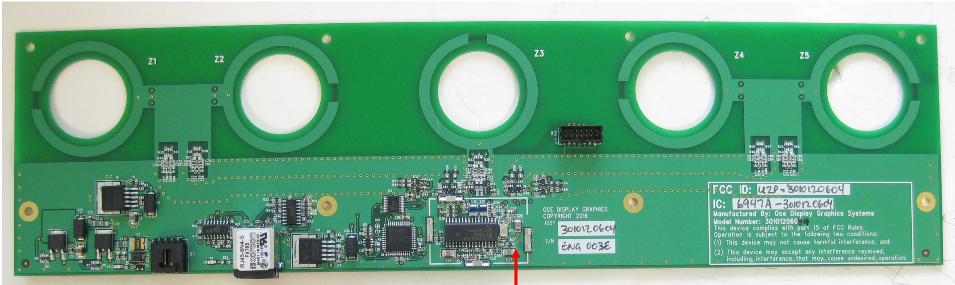
Figure 2: 3010120604 RFID Reader Front Side – RF Shield is removed.
