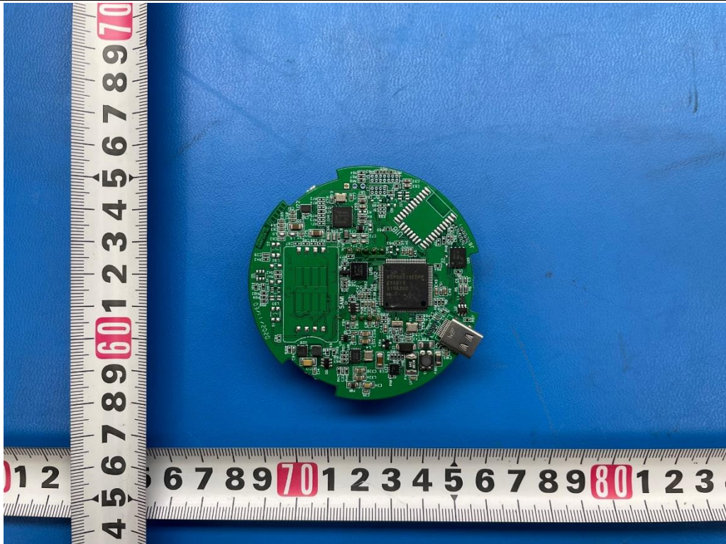
Internal Bottom Board Rear View
