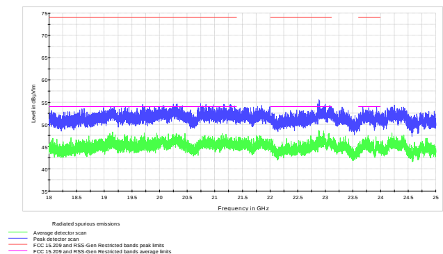
Figure 8.7-27: Radiated spurious emissions above 18 GHz for \pi/4 -DQPSK modulation low channel
