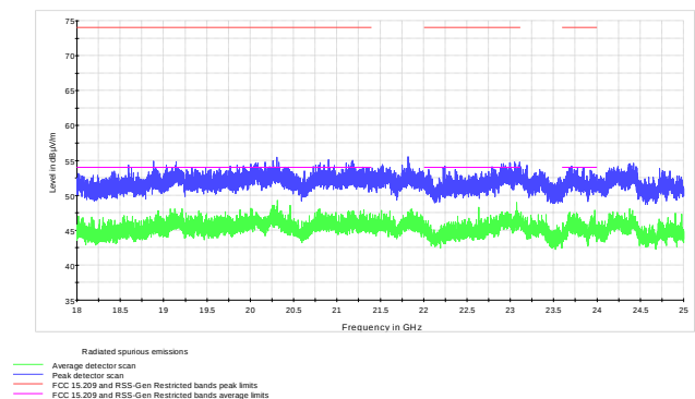
Figure 8.7-21: Radiated spurious emissions above 18 GHz for GFSK modulation mid channel
