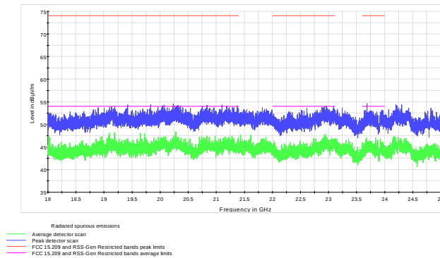
Figure 8.7-42: Radiated spurious emissions above 18 GHz for 8-DPSK modulation high channel
