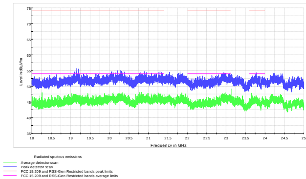
Figure 8.7-36: Radiated spurious emissions above 18 GHz for 8-DPSK modulation low channel
