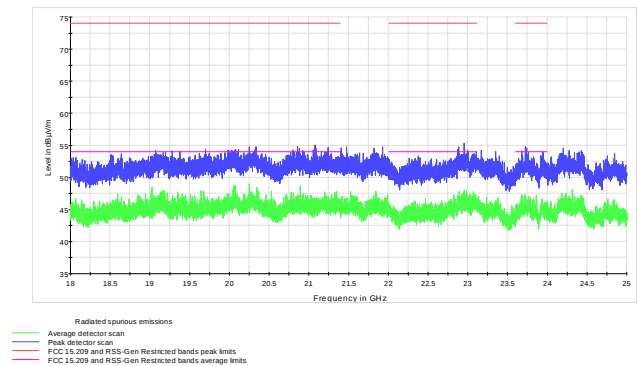
Figure 8.7-33: Radiated spurious emissions above 18 GHz for \pi/4 -DQPSK modulation high channel
