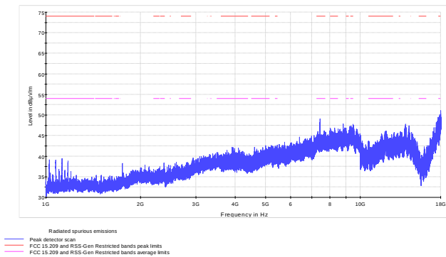
Figure 8.7-38: Radiated spurious emissions within 1–18 GHz for 8-DPSK modulation mid channel
