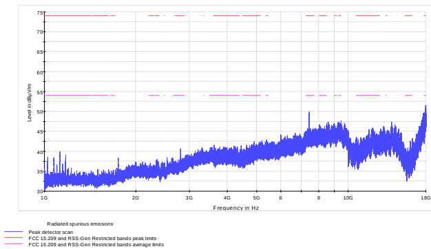
Figure 8.7-32: Radiated spurious emissions within 1–18 GHz for \pi/4 -DQPSK modulation high channel
