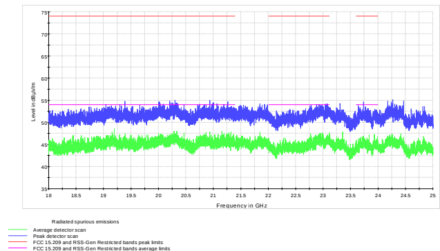
Figure 8.7-39: Radiated spurious emissions above 18 GHz for 8-DPSK modulation mid channel
