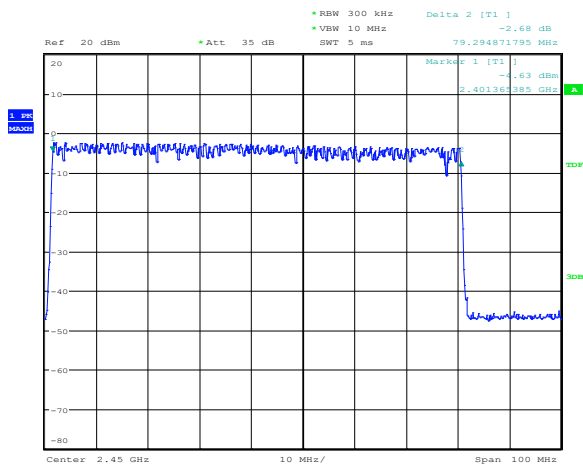
Figure 8.5-1: 20 dB bandwidth sample plot
