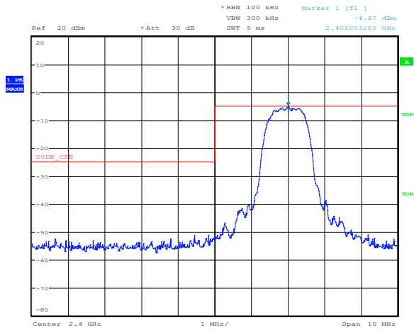
Figure 8.7-1: Band edge spurious emissions at 2400 MHz for GFSK modulation
