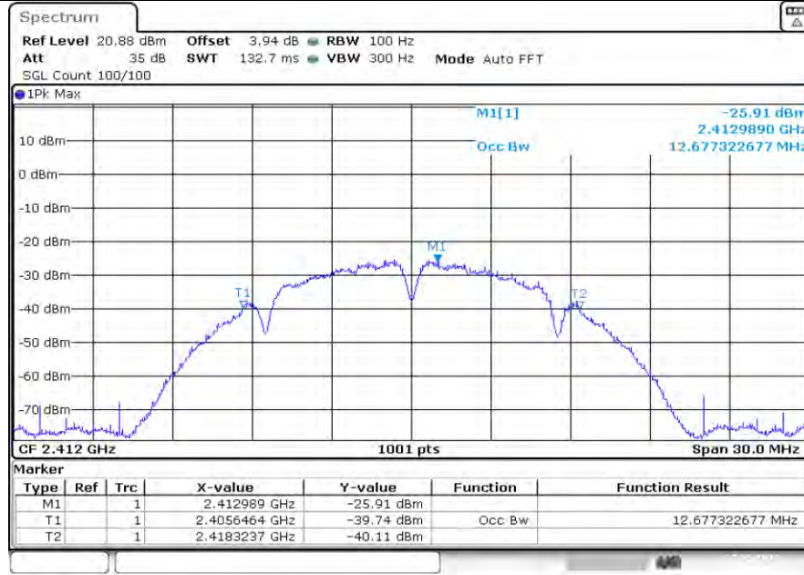
99%_Occupied_Bandwidth_NVNT_ANT1_802_11b_2412
