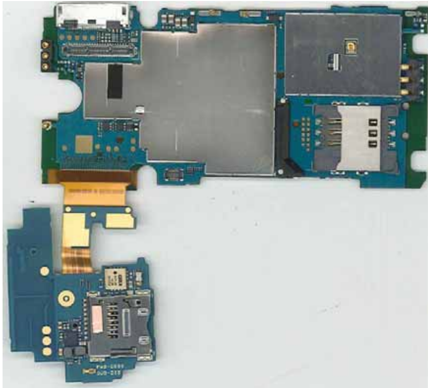
SHIELD COVER put on MAIN PCB
