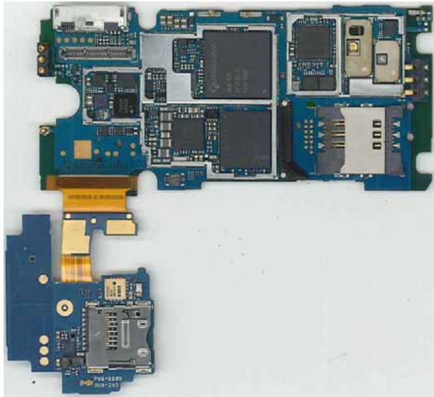
MAIN PCB (TOP VIEW) & SUB (BOTTOM VIEW) with Shield Frame & Cushion
