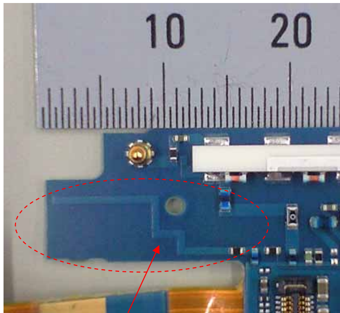
Bluetooth Pattern Antenna
