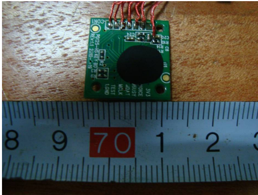
EUT – Keyboard TopView (Handset)
