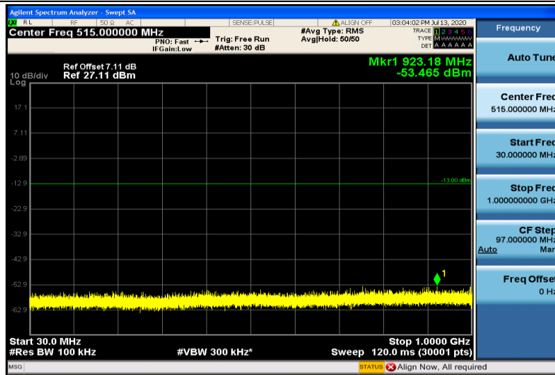
Band2-5MHz-QPSK-18900-1RB#0-30~1000MHz
