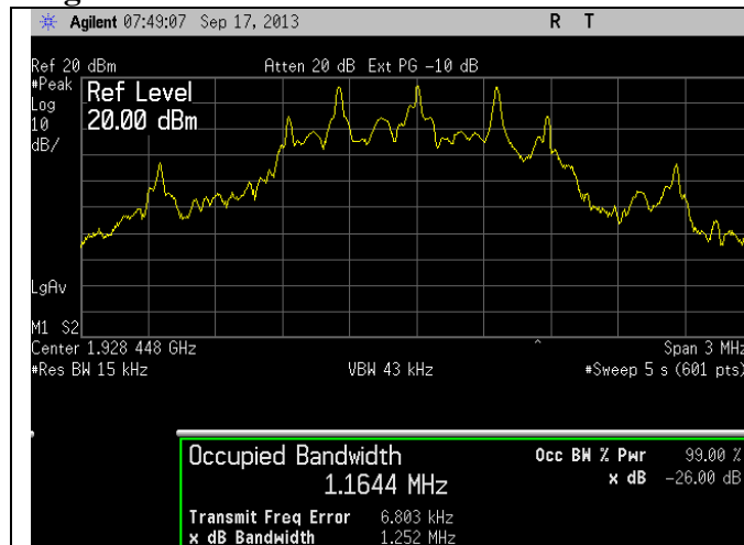
Antenna 0
