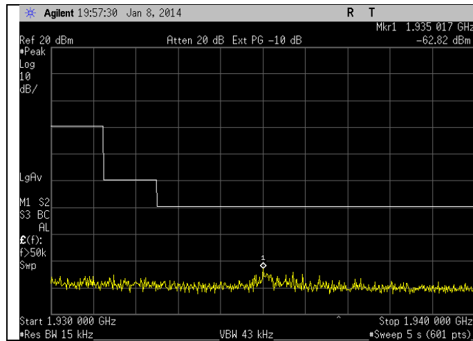
Antenna 0
