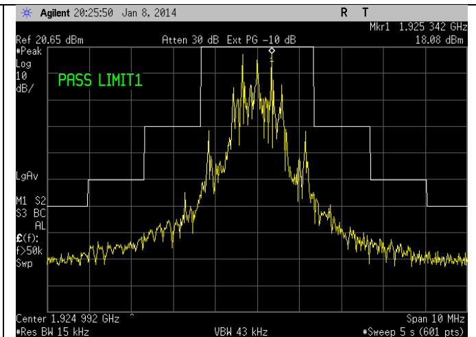
Antenna 1
