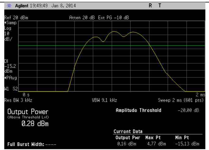
PSD
