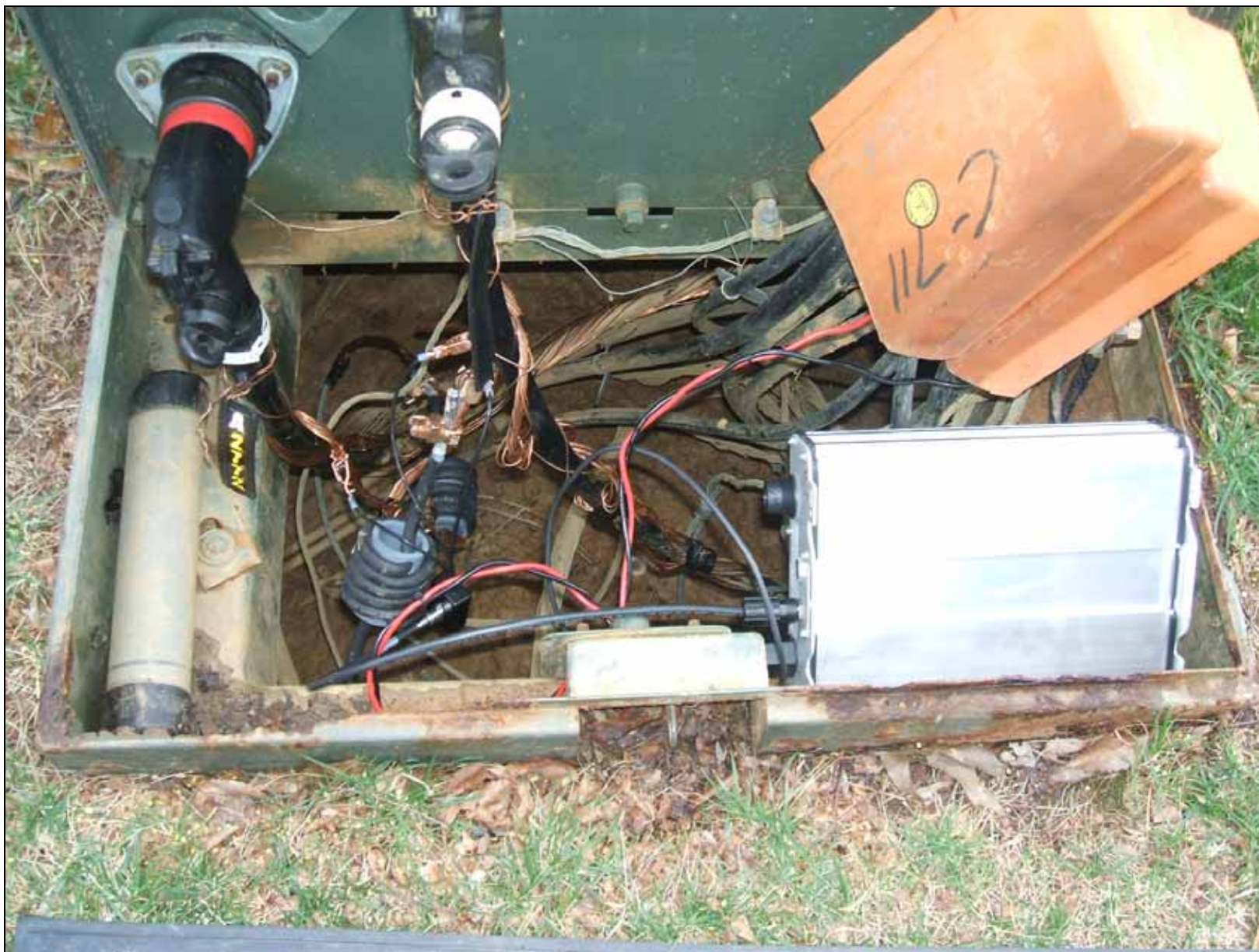
Photograph B-6: Test Site Photo – CURRENT Group Gaithersburg Test Area – A-7042 (open case)
