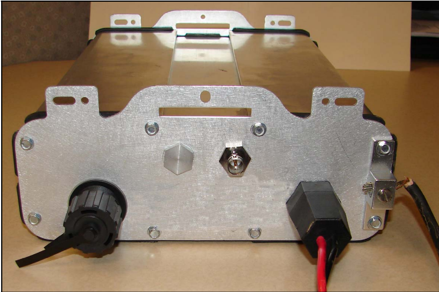
Photograph EP-3: External Photo of CURRENT Bridge URD 6121 – View from bottom of unit
