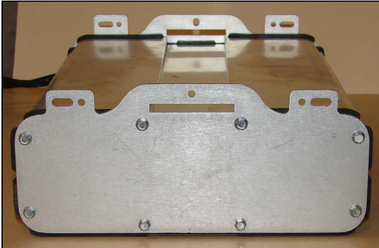
Photograph EP-2: External Photo of CURRENT Bridge URD 6121 – View from top of unit
