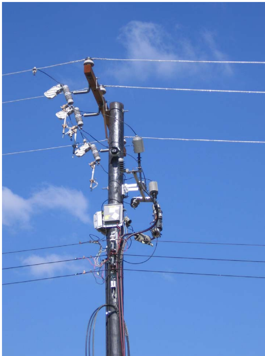
Photograph B-4: Radiated Emissions Test – CURRENT Technologies Field Research and Test Area, Pole P4- Close View
