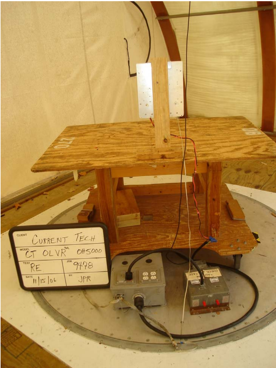
Photograph B-2: Radiated Emissions Test – Washington Laboratories OATS – Rear View
