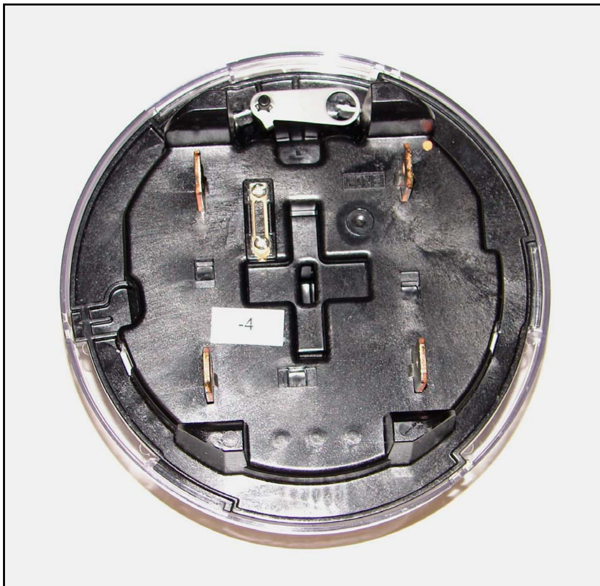
Photograph EP-2: External Photo of CT AMR Meter – View of Bottom Side
