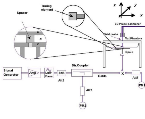
Fig 8.3.1 System Performance Check Setup
