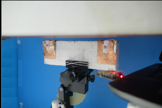
Left Side of Antenna Mode Tested at 5 mm
