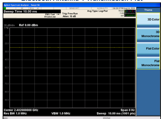
Bluetooth Antenna-1 Transmission Plot
