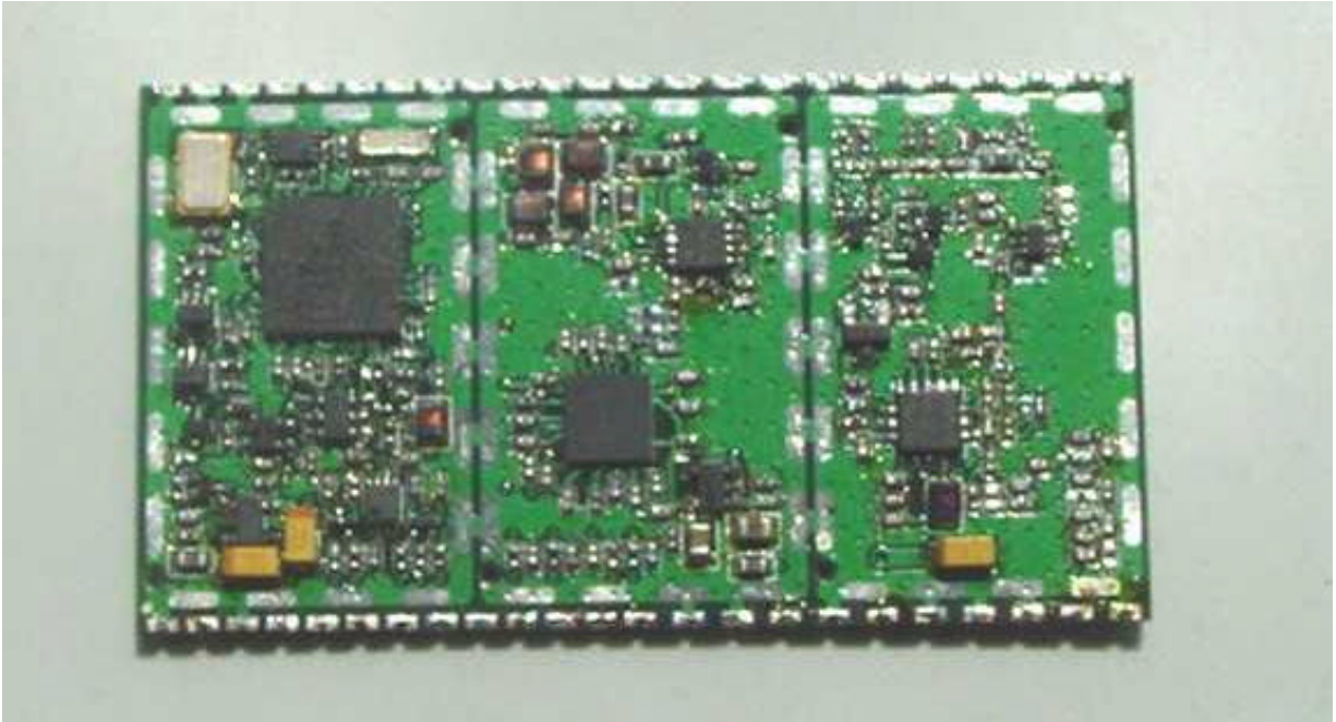
Transmitter Board Top, RF Shields Removed
