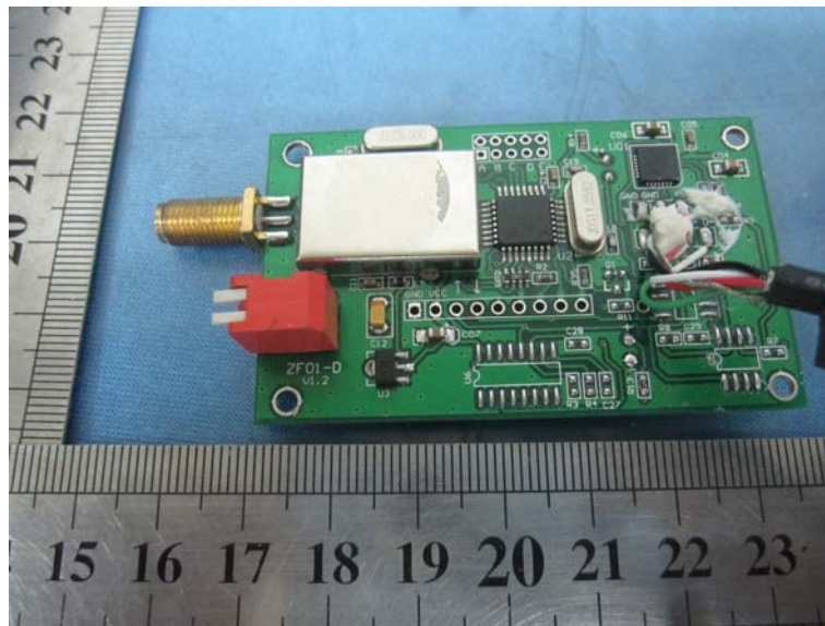
The photo of IC:mega8 PCB board
