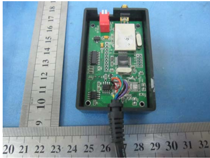
RS422 port
