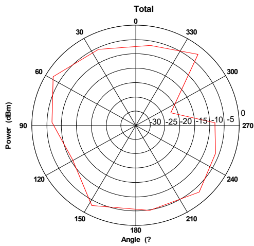
XZ Plane at f = 0.315GHz
