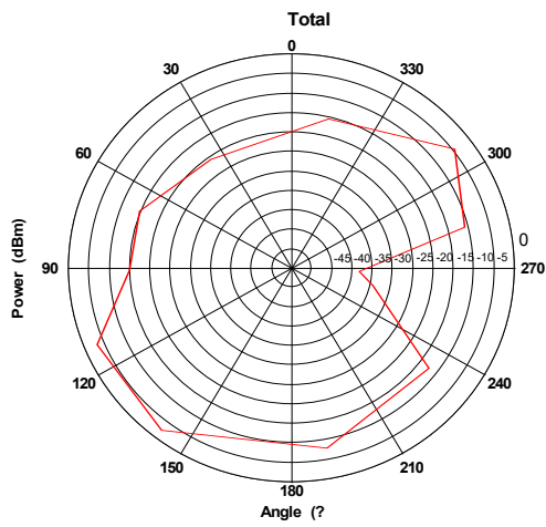
XY Plane at f = 0.315GHz
