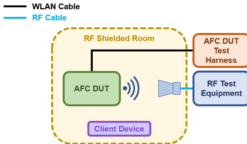
Standard Power Access Points Test Setup
