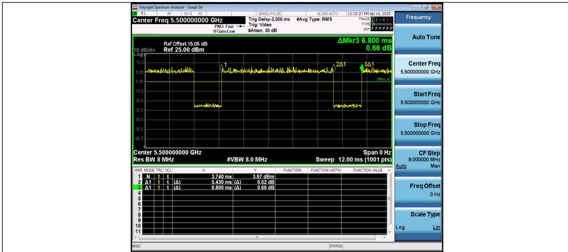
NTNV-11AC20MIMO-Ant1-5500
