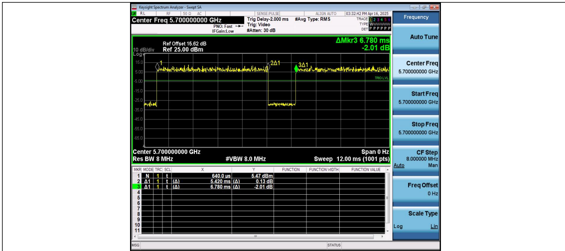
NTNV-11AC20MIMO-Ant2-5700
