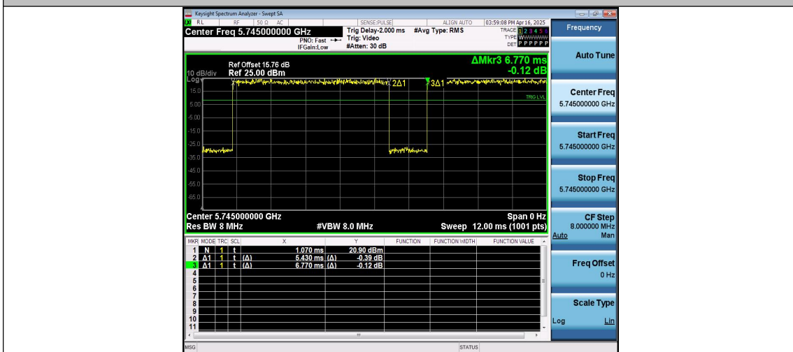
NTNV-11AC20MIMO-Ant3-5745
