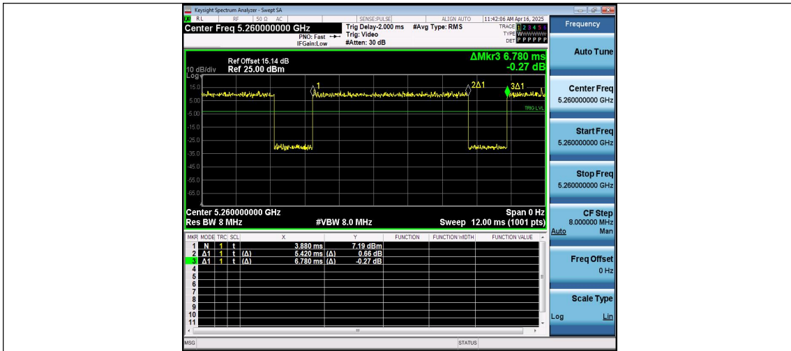
NTNV-11AC20MIMO-Ant4-5260
