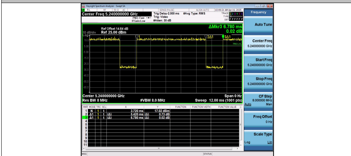
NTNV-11AC20MIMO-Ant1-5240
