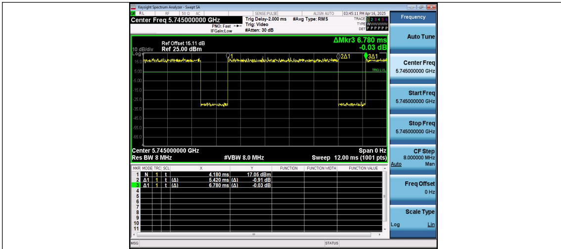
NTNV-11AC20MIMO-Ant1-5745
