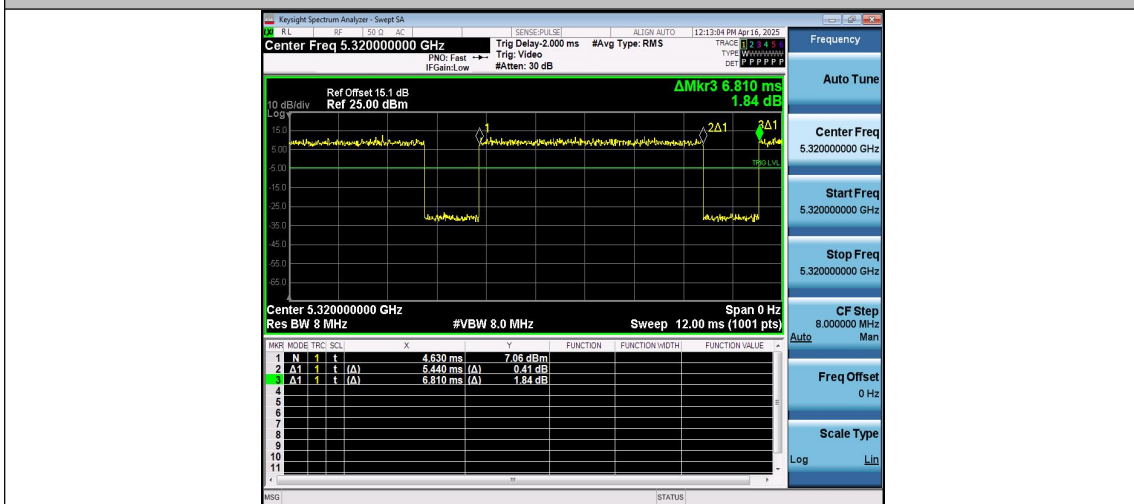
NTNV-11AC20MIMO-Ant1-5320
