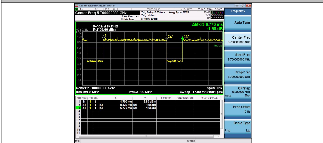
NTNV-11AC20MIMO-Ant4-5700
