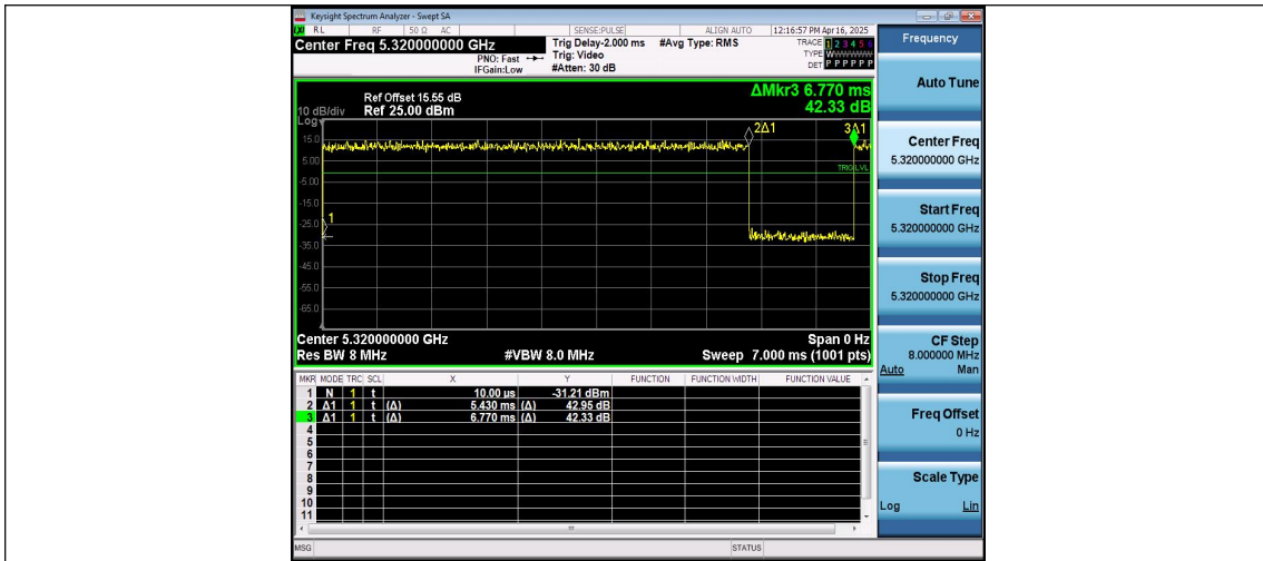
NTNV-11AC20MIMO-Ant2-5320
