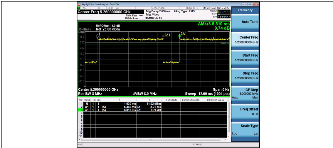
NTNV-11AC20MIMO-Ant1-5260
