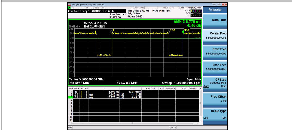
NTNV-11AC20MIMO-Ant2-5500
