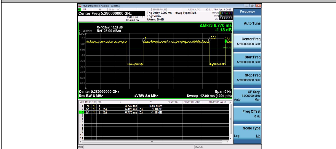
NTNV-11AC20MIMO-Ant2-5280
