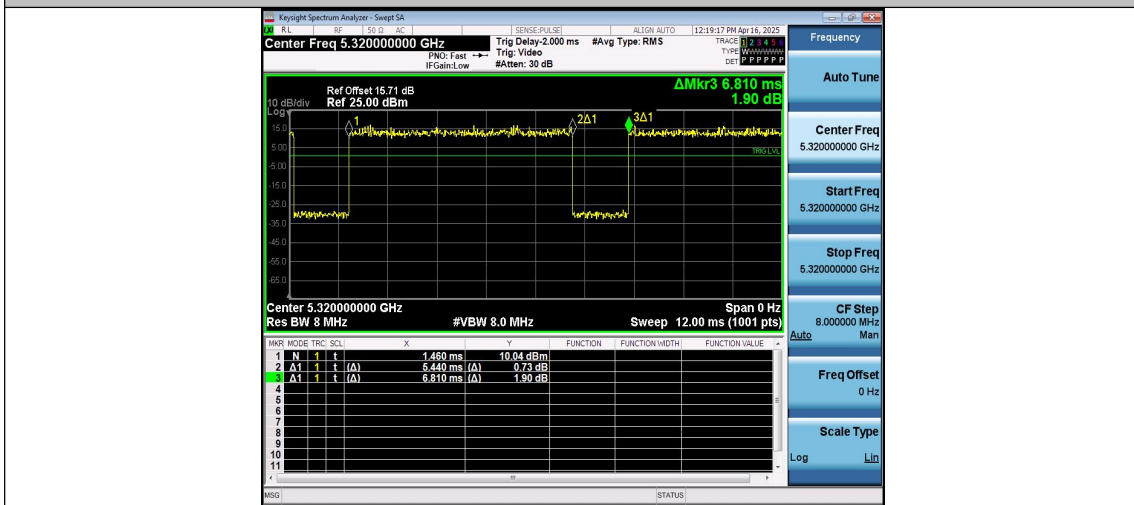
NTNV-11AC20MIMO-Ant3-5320
