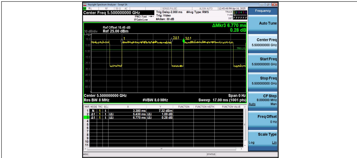
NTNV-11AC20MIMO-Ant4-5500
