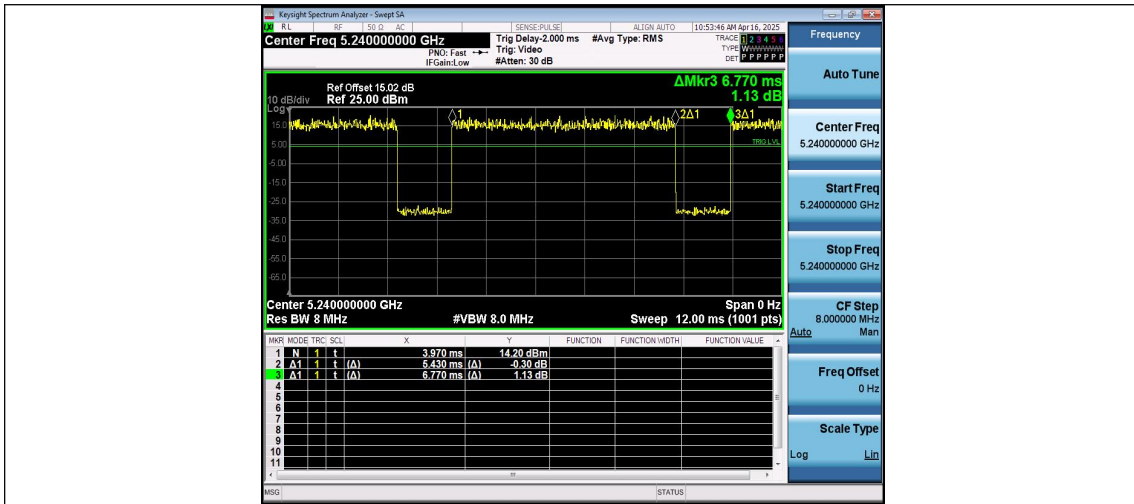
NTNV-11AC20MIMO-Ant2-5240
