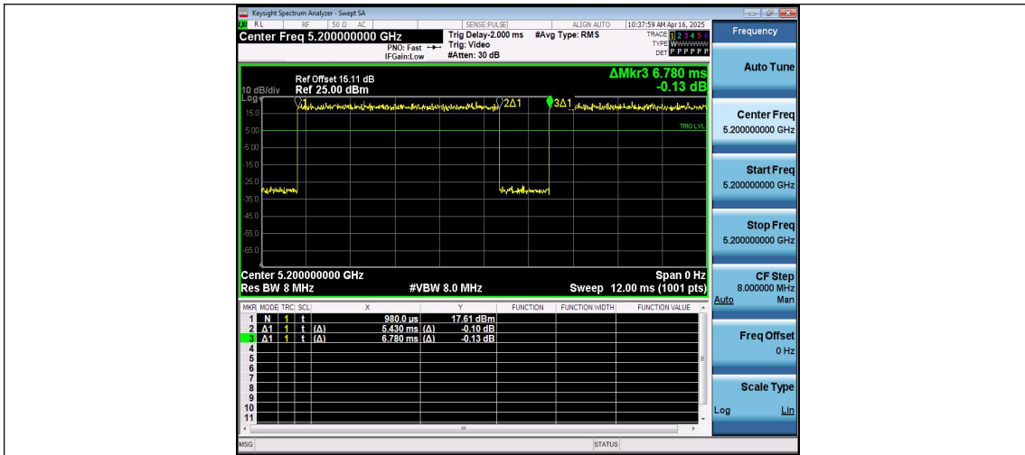
NTNV-11AC20MIMO-Ant3-5200
