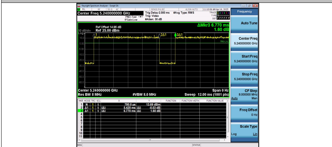
NTNV-11AC20MIMO-Ant4-5240
