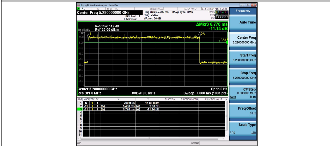
NTNV-11AC20MIMO-Ant1-5280
