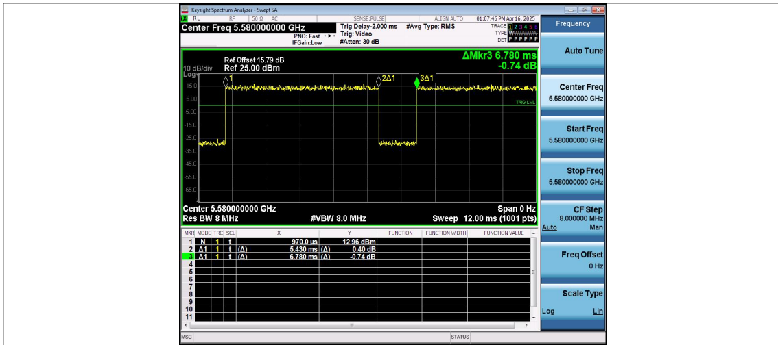
NTNV-11AC20MIMO-Ant3-5580
