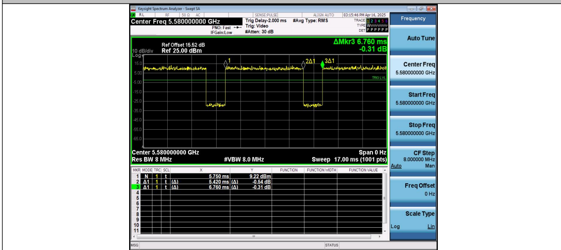
NTNV-11AC20MIMO-Ant4-5580
