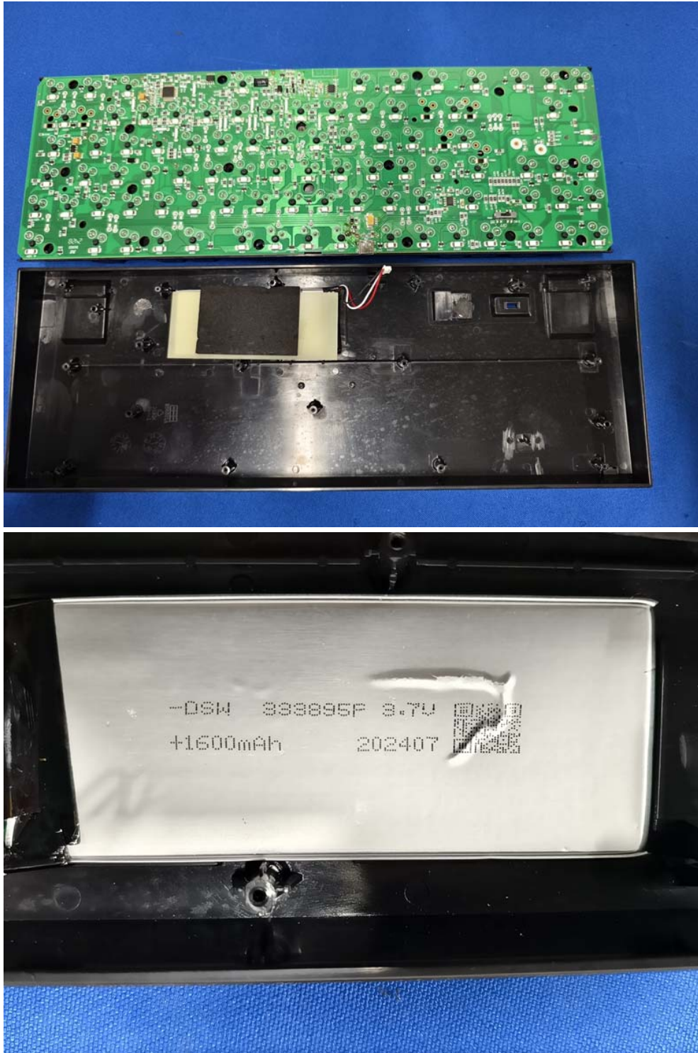
Inside View-Keybord
