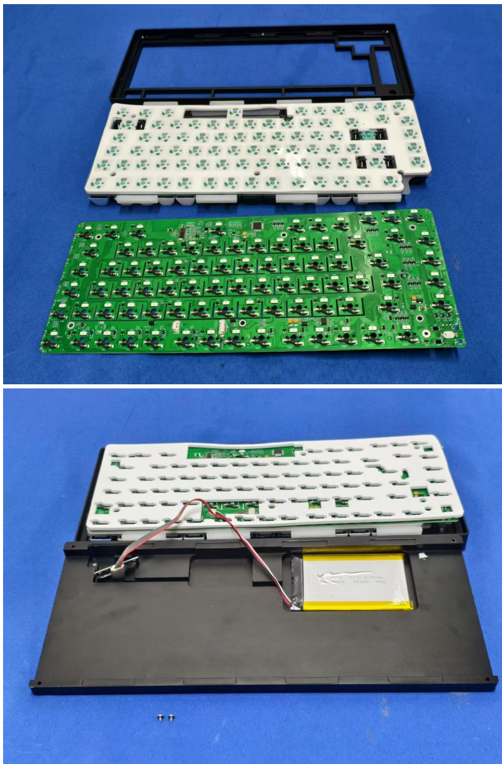
Inside View-Keybord
