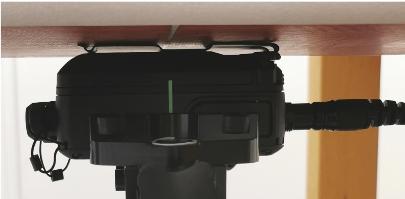
Figure 8 Back side of the DUT against the phantom, 0mm separation distance
