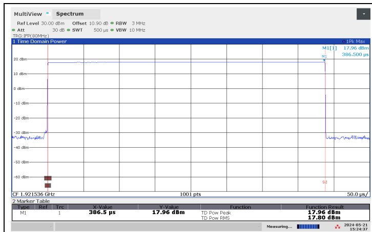
Conducted Peak Output Power, Lower Channel
