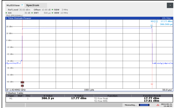
Conducted Peak Output Power, Middle Channel
