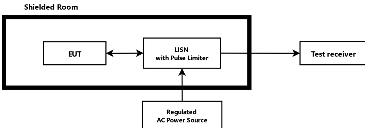
Test Set-Up 4
