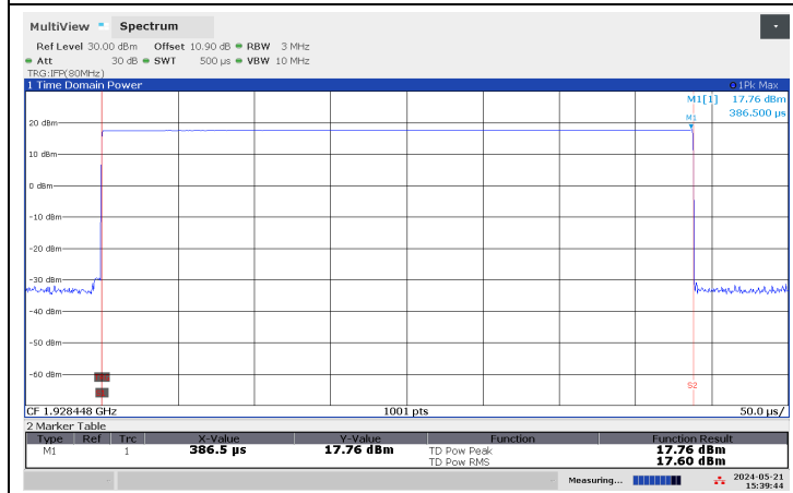
Conducted Peak Output Power, Upper Channel
