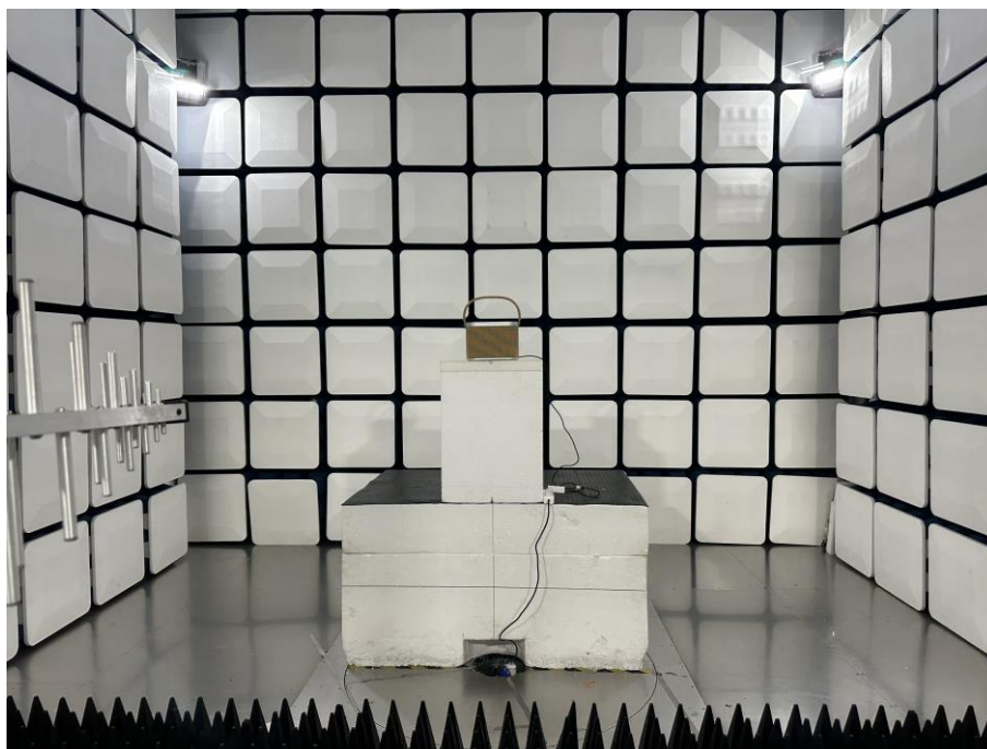
960MHz-1GHz
