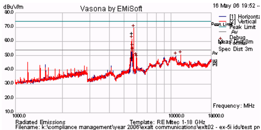
5,745 MHz Radiated Emissions for 37.9 dBi Antenna 30 MHz Bandwidth QPSK
