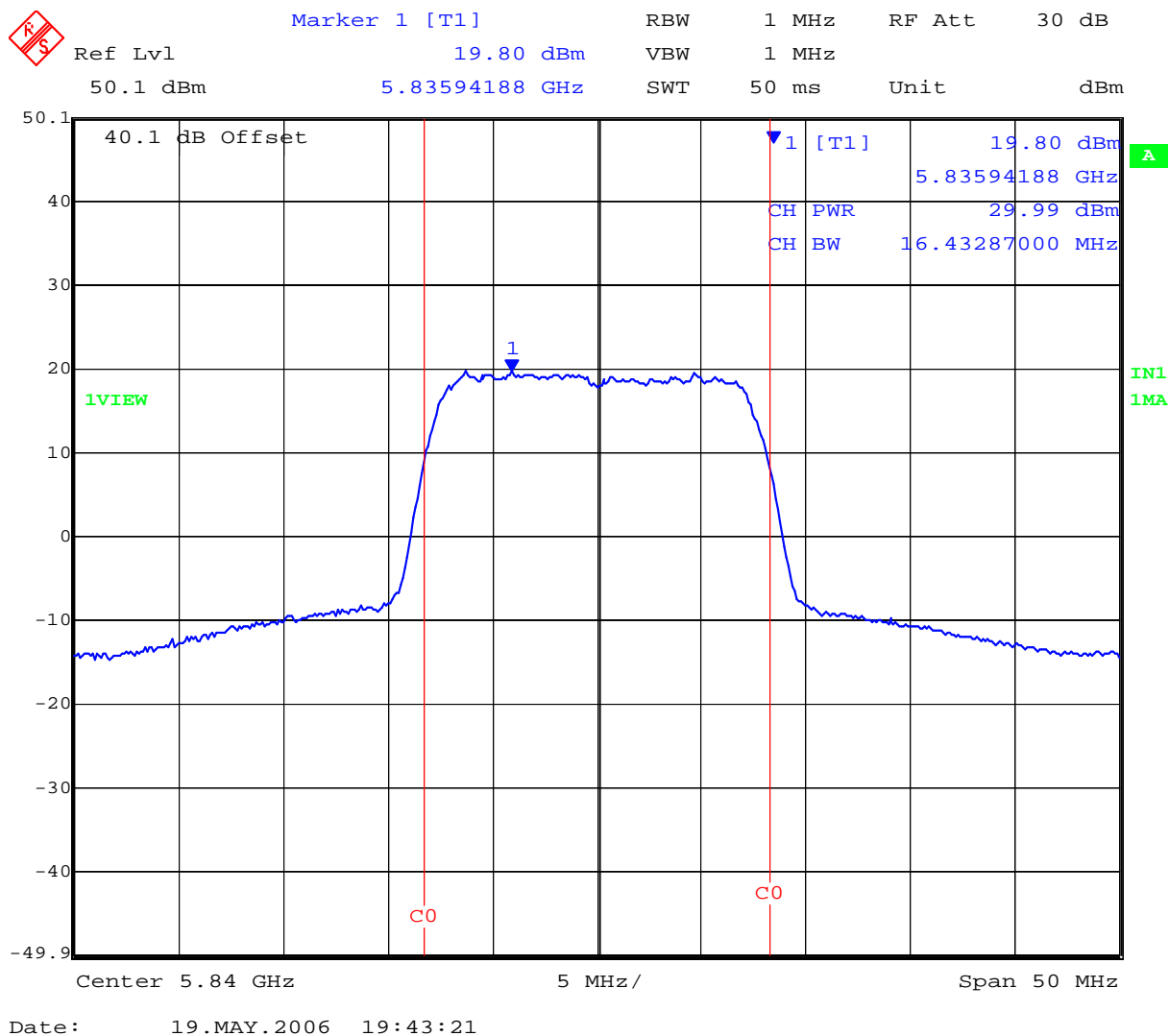
Plot 06 5,840 MHz 15 MHz QPSK Peak Power (dBm)
