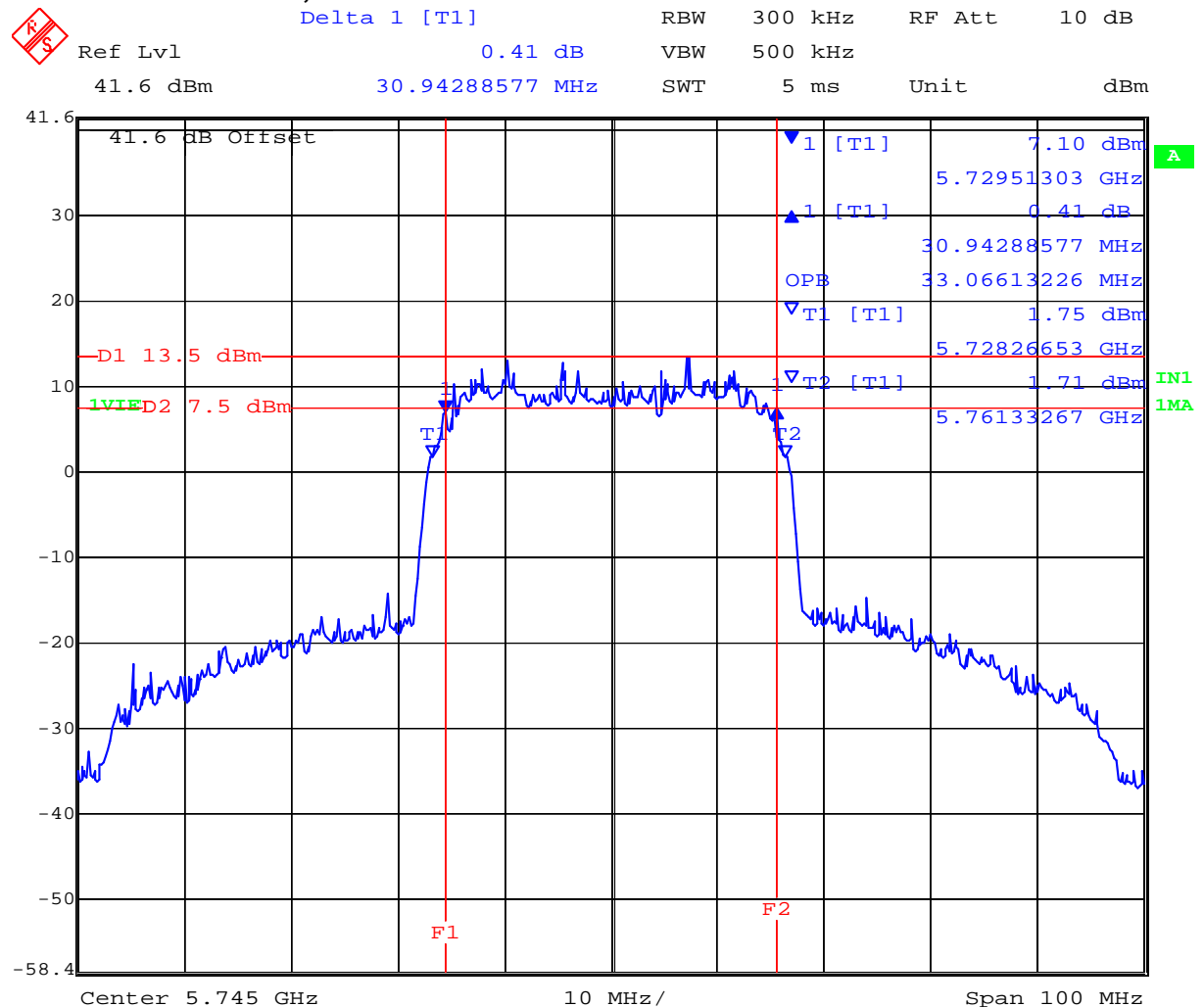
Plot 03 5,745 MHz 30 MHz QPSK 6 dB& 99% Bandwidth
