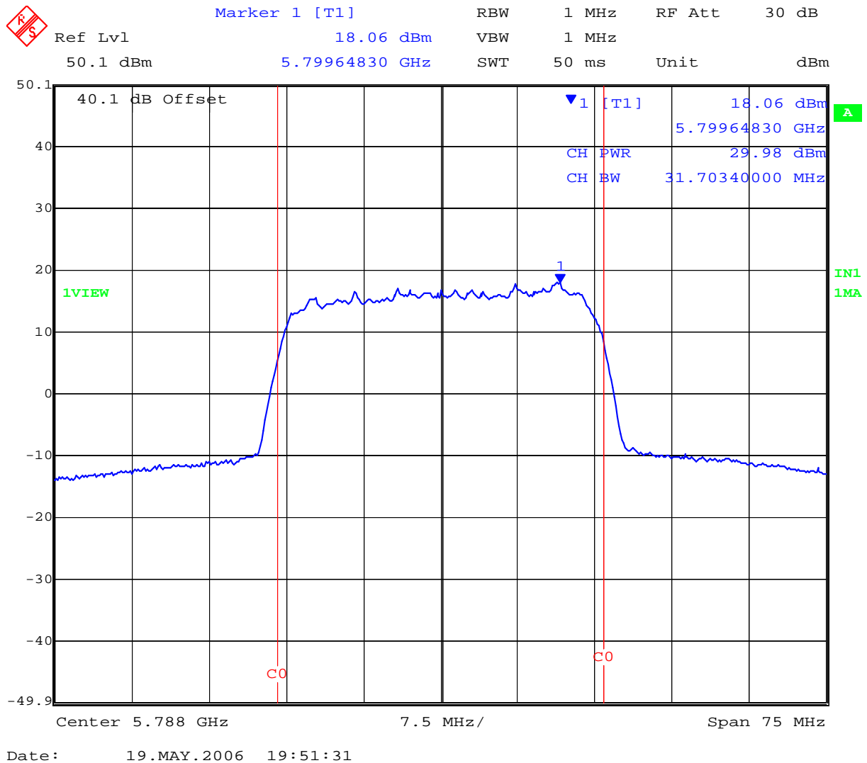
Plot 07 5,788 MHz 30 MHz QPSK Peak Power (dBm)
