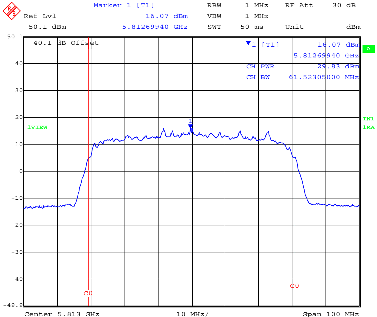
Plot 08 5,813 MHz 60 MHz QPSK Peak Power (dBm)
