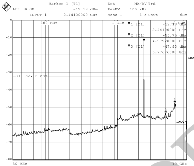
(a) Frequency Range: 30 MHz to 10 GHz
