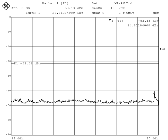
(c) Frequency Range: 18 GHz to 25 GHz
