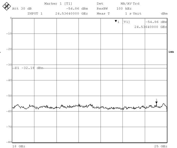
(c) Frequency Range: 18 GHz to 25 GHz
