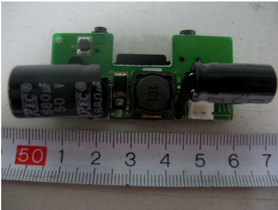
Power Board Top Components View
