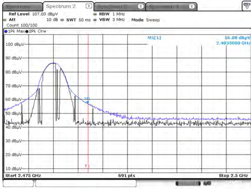
Radiated Restricted Band Edges plot – Average & Peak Reading (8DPSK, Ch.78, X-H)
