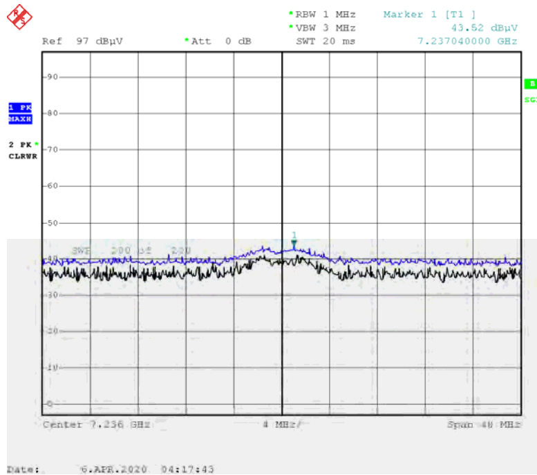
Radiated Spurious Emissions plot – Peak Reading (802.11b, Ch.1 3rd Harmonic, X-V)
