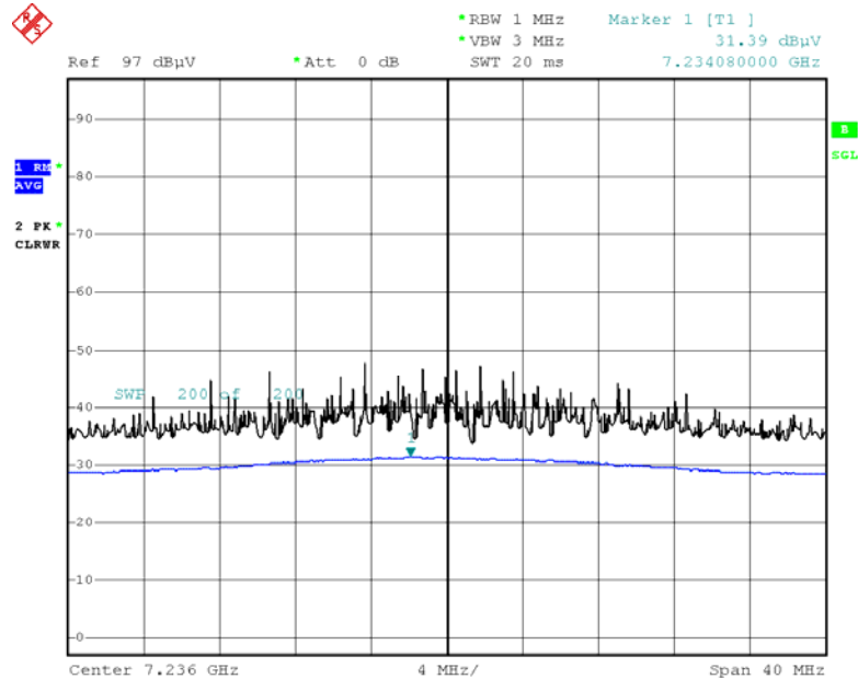
Radiated Spurious Emissions plot – Average Reading (802.11g, Ch.1 3rd Harmonic, V)
