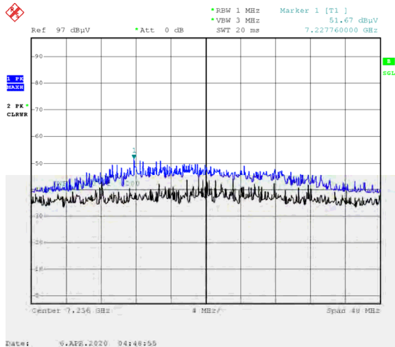
Radiated Spurious Emissions plot – Peak Reading (802.11n (HT20), Ch.1 3rd Harmonic, V)
