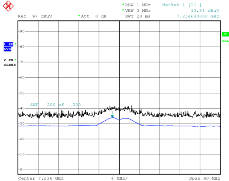
Radiated Spurious Emissions plot – Average Reading (802.11b, Ch.1 3rd Harmonic, X-V)
