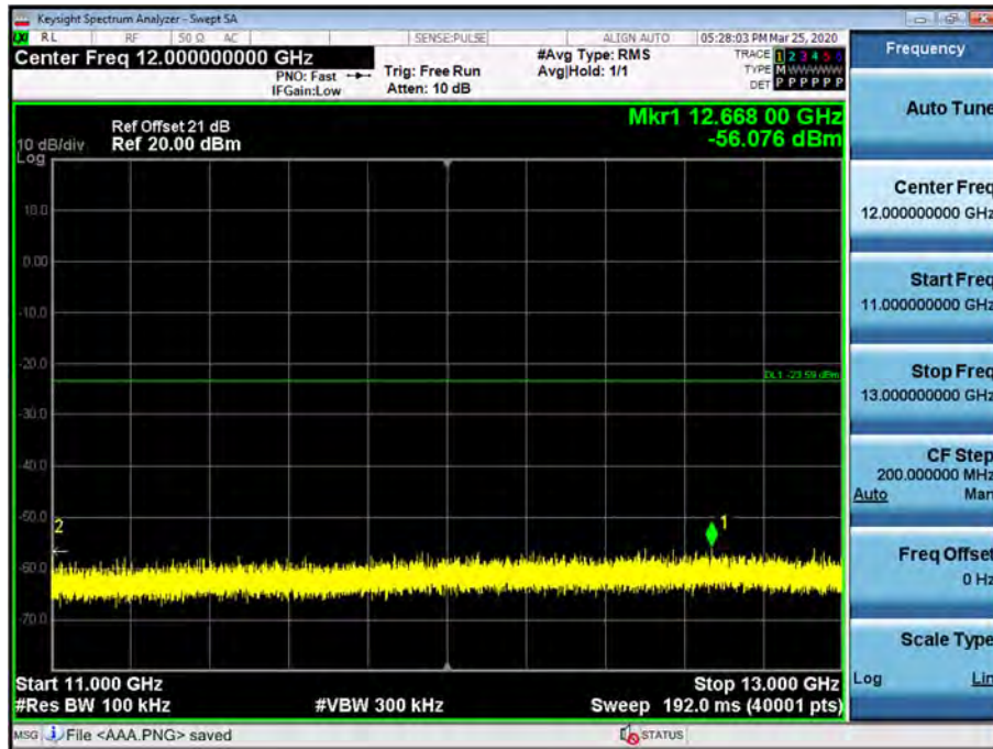
Conducted Spurious Emission (802.11b_Ch.11_MCS6)
