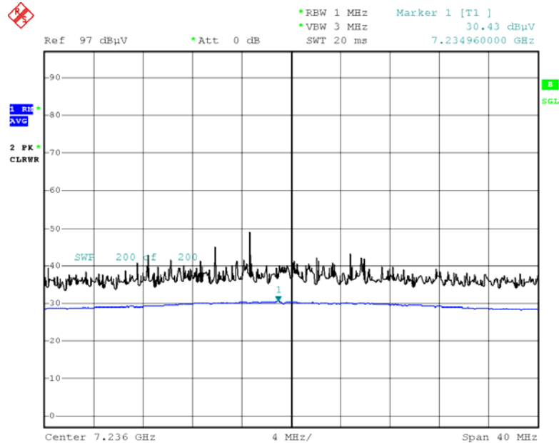
Radiated Spurious Emissions plot – Average Reading (802.11n (HT20), Ch.1 3rd Harmonic, V)
