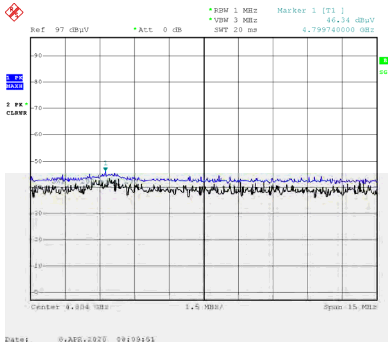
Radiated Spurious Emissions plot – Peak Reading (GFSK, Ch.0 2nd Harmonic, X-V)
