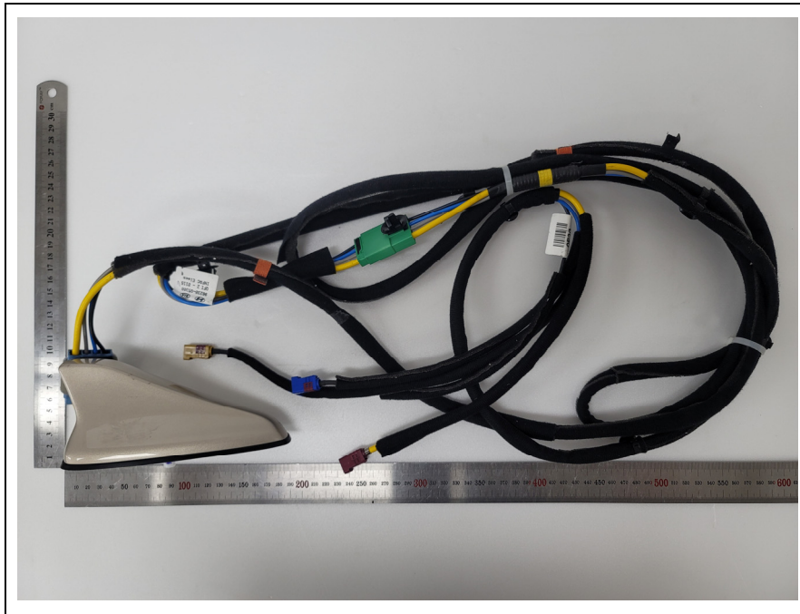
<Shark Antenna>
