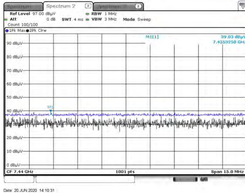
Radiated Spurious Emissions plot – Average &amp; Peak Reading (8DPSK, Ch.78 3rd Harmonic, X-H)
