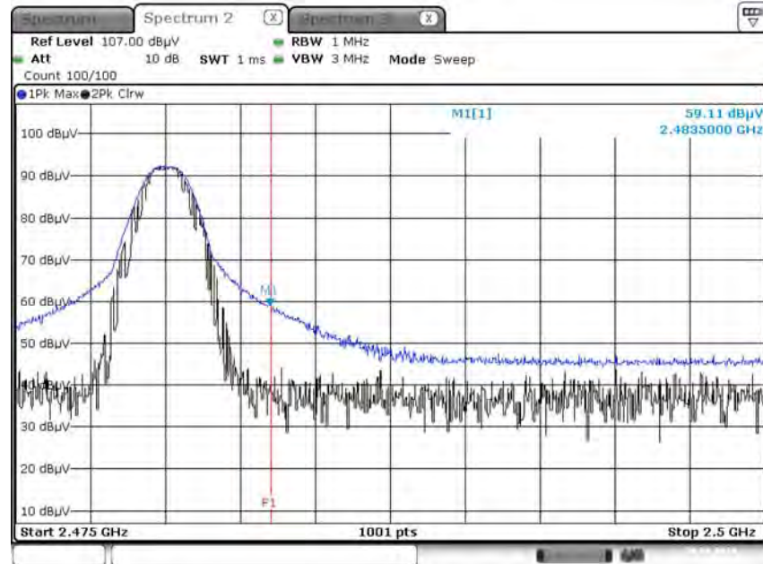
Radiated Restricted Band Edges plot – Average &amp; Peak Reading (GFSK, Ch.78, X-H)
