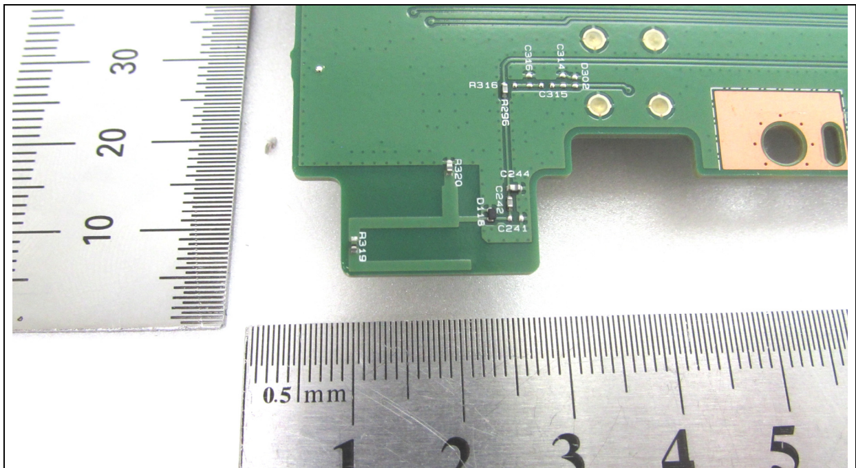
<BT Antenna>
