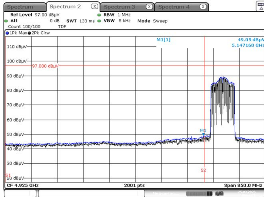
Average Result (802.11 ac_VHT80_ MCS0, Ch.42, X-H)
