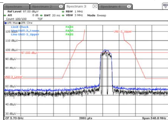
Peak Result (802.11ac_VHT40, Ch.159, X-H)
