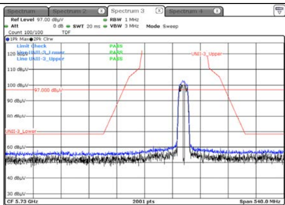
Peak Result (802.11n_HT20, Ch.161, X-H)
