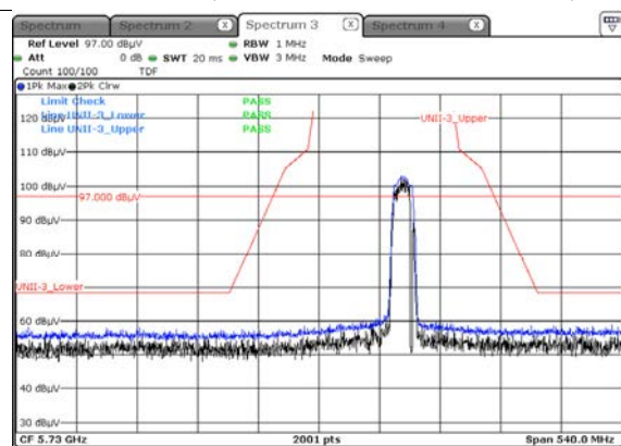
Peak Result (802.11ac_VHT20, Ch.161, X-H)
