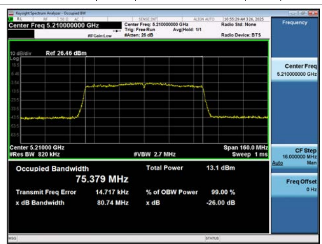
802.11ac(VHT80) 26 dB Bandwidth (CH 42)
