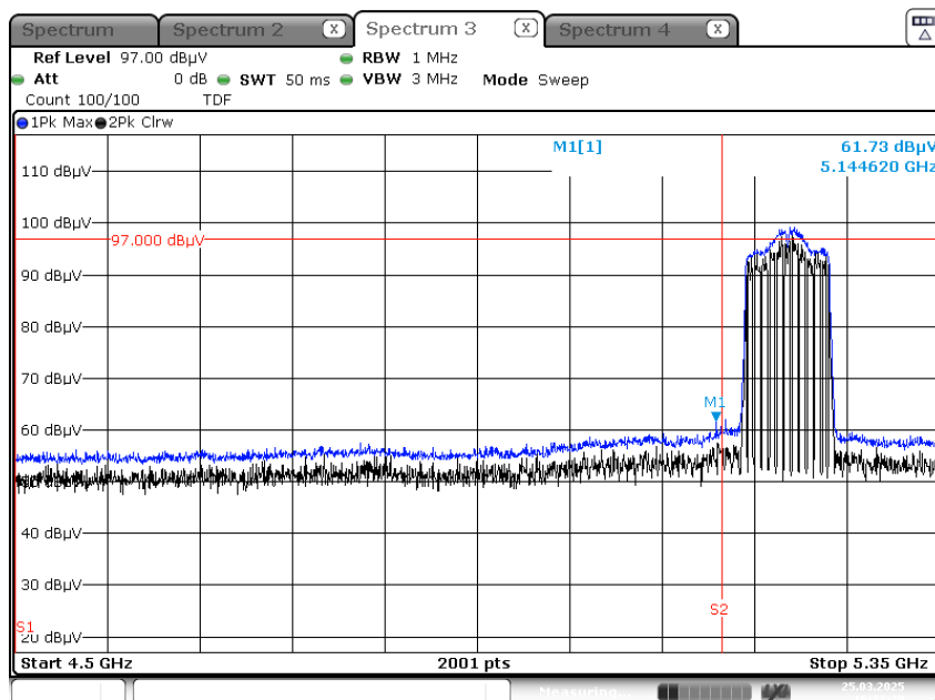
Peak Result (802.11 ac_VHT80_ MCS0, Ch.42, X-H)
