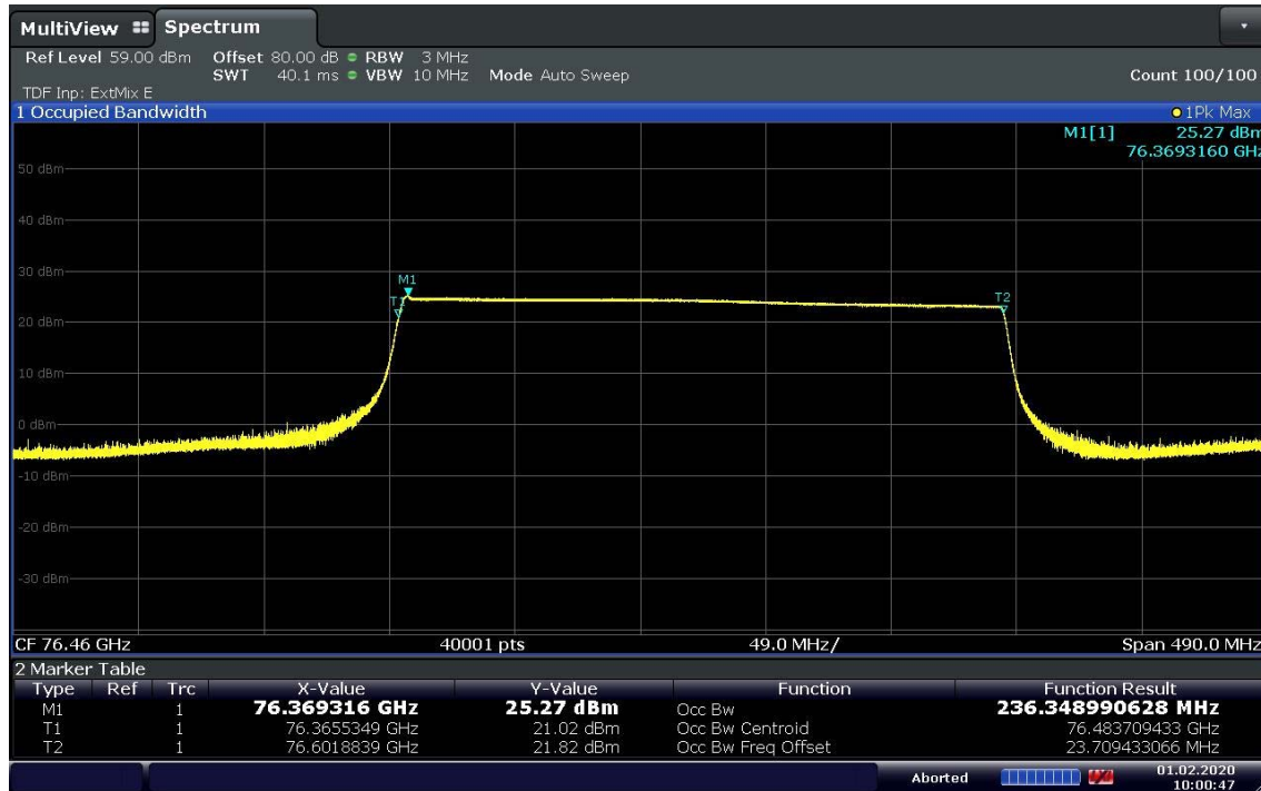
Occupied Bandwidth plot (High Resolution)
