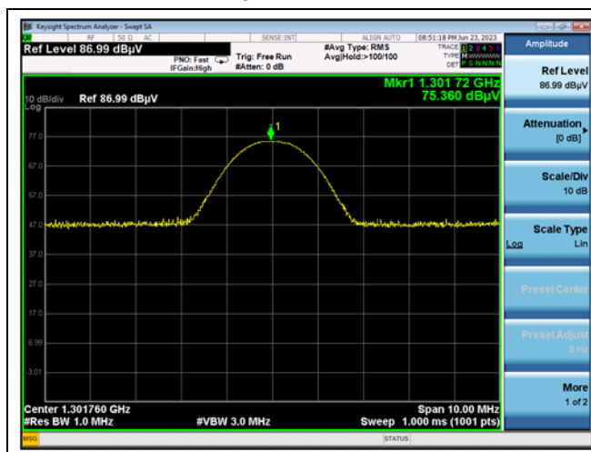
3 rd harmonic
