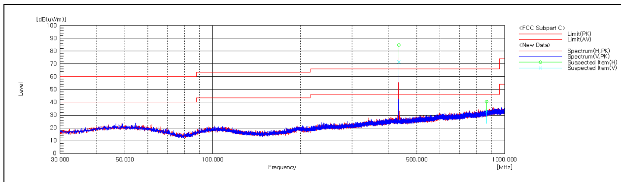
3 rd harmonic
