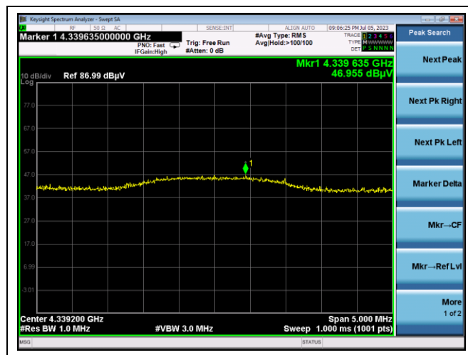
10 th harmonic
