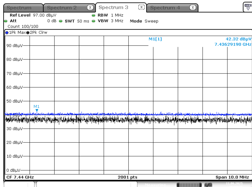
Radiated Spurious Emissions plot – Peak Result (3rd Harmonic)
