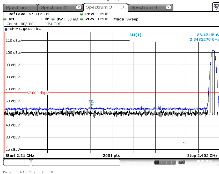
Radiated Restricted Band Edges plot – Peak Result (Ch.0, Z-V)
