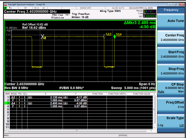
1 M Bit/s (255 Byte) Duty Cycle (Low-CH 0)
