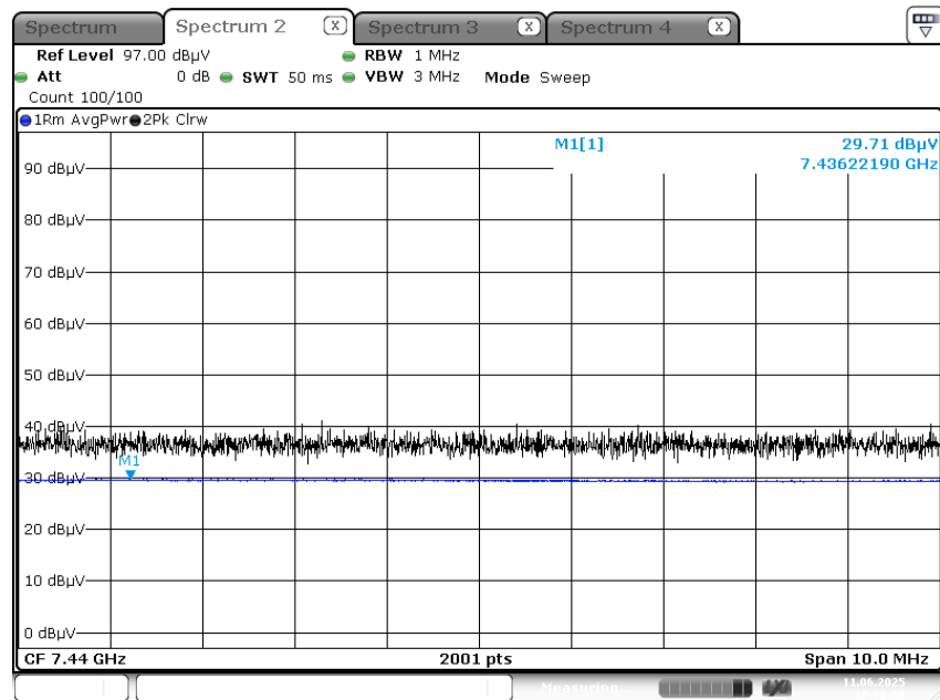
Radiated Spurious Emissions plot – Average Result (3rd Harmonic)
