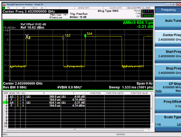
1 M Bit/s (37 Byte) Duty Cycle (Low-CH 0)
