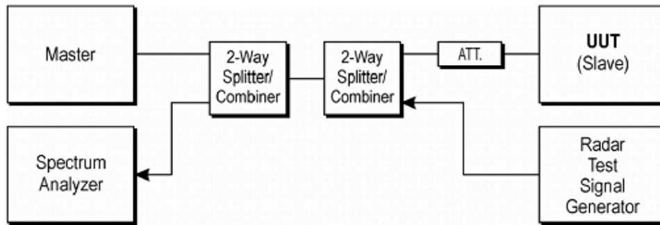
Figure 7-1. Test Setup
