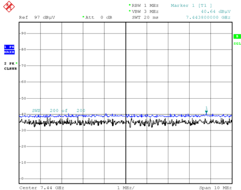
Radiated Spurious Emissions plot – Peak Reading ( \pi /4QPSK, Ch.78 3rd Harmonic)
