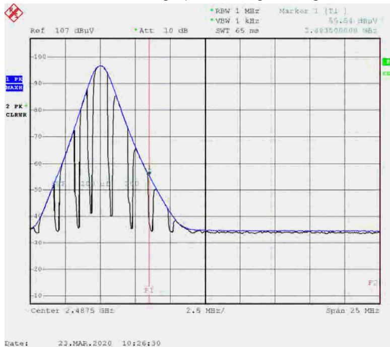
Radiated Restricted Band Edges plot – Peak Reading (GFSK, Ch.78)
