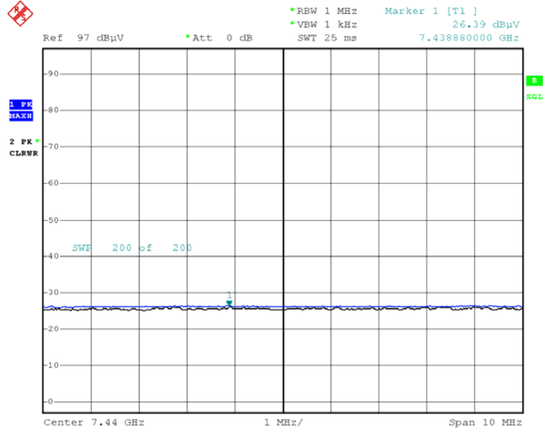
Radiated Spurious Emissions plot – Average Reading ( \pi /4QPSK, Ch.78 3rd Harmonic)
