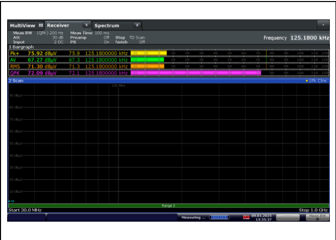
AST Antenna
