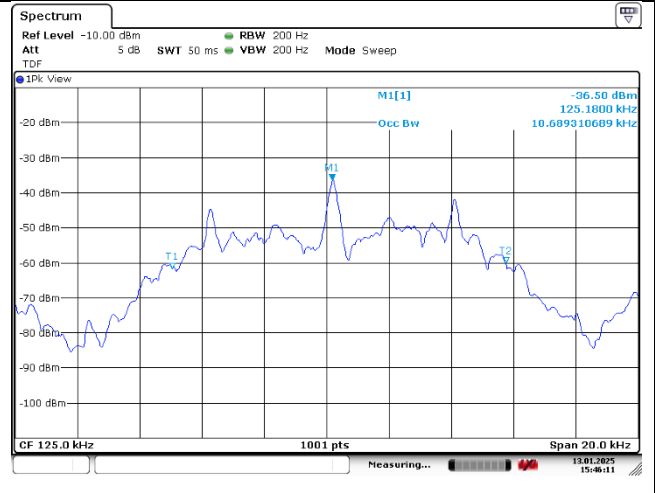
INT2 Antenna
