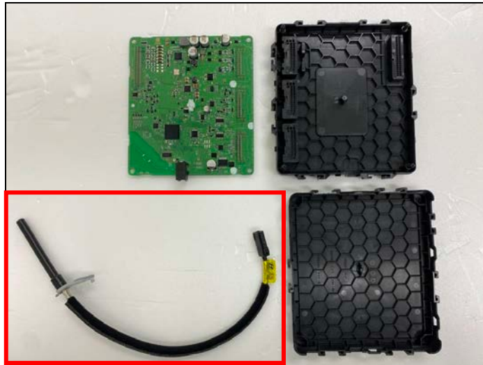
Receive Antenna
