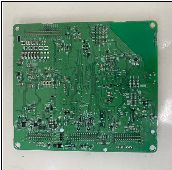
Bottom view of Main PCB
