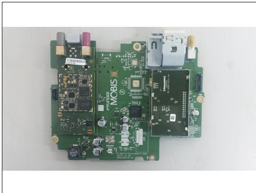
Top view of Sub1 PCB (with LTE, CDMA modem)
