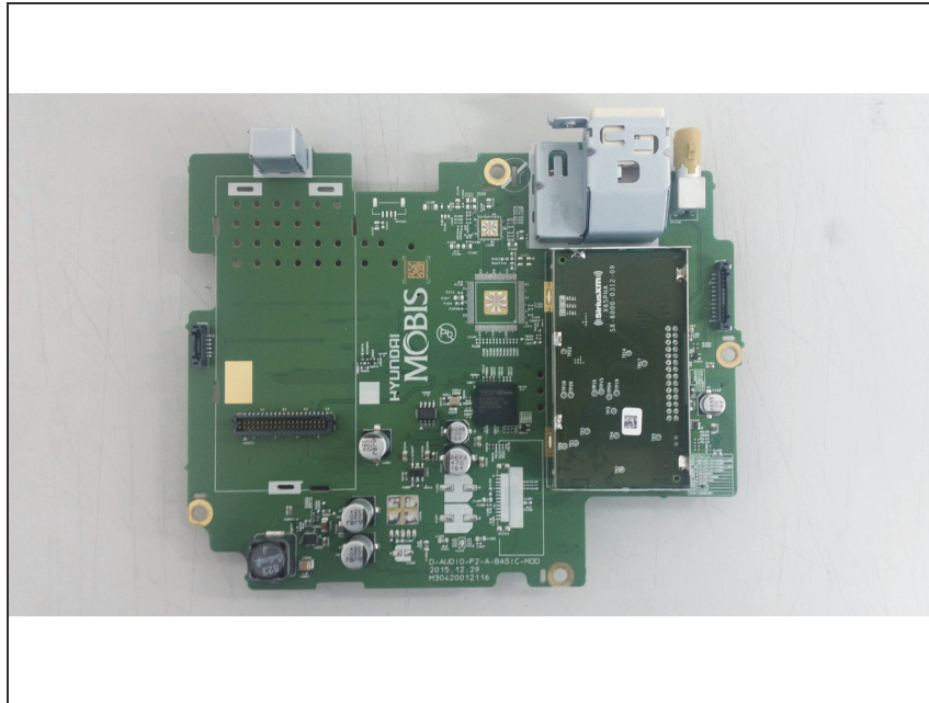
Top view of Sub1 PCB (without LTE, CDMA modem)
