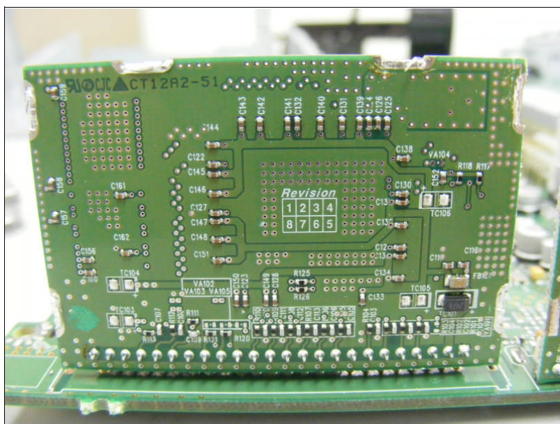
Bottom view of Sub Board#3
