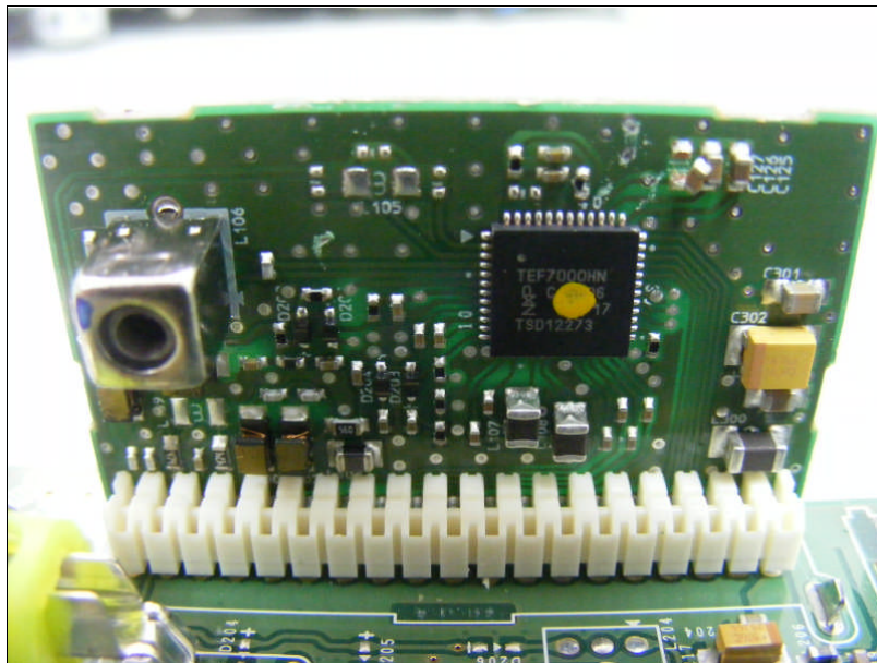
Bottom view of Sub Board#4
